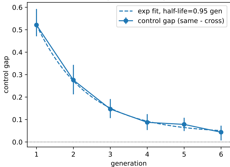
Decay (class=decay)
