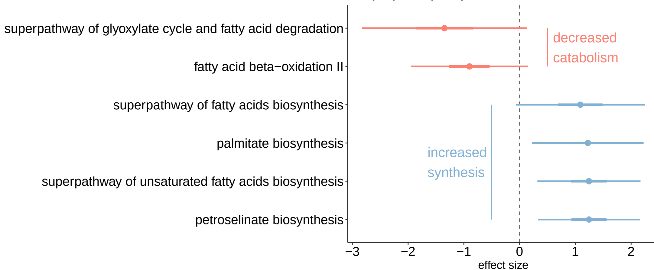
A. Lipid pathway temperature coefficients
