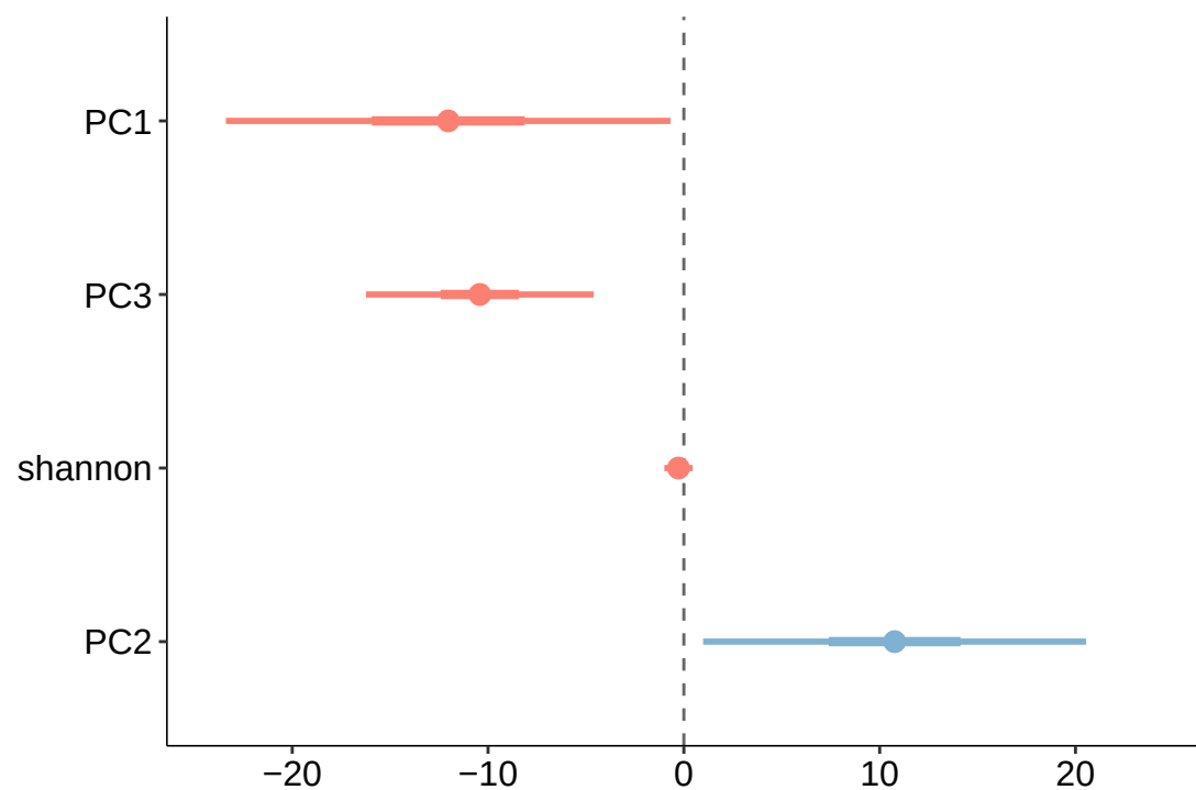
Metabolic pathway temperature coefficients
