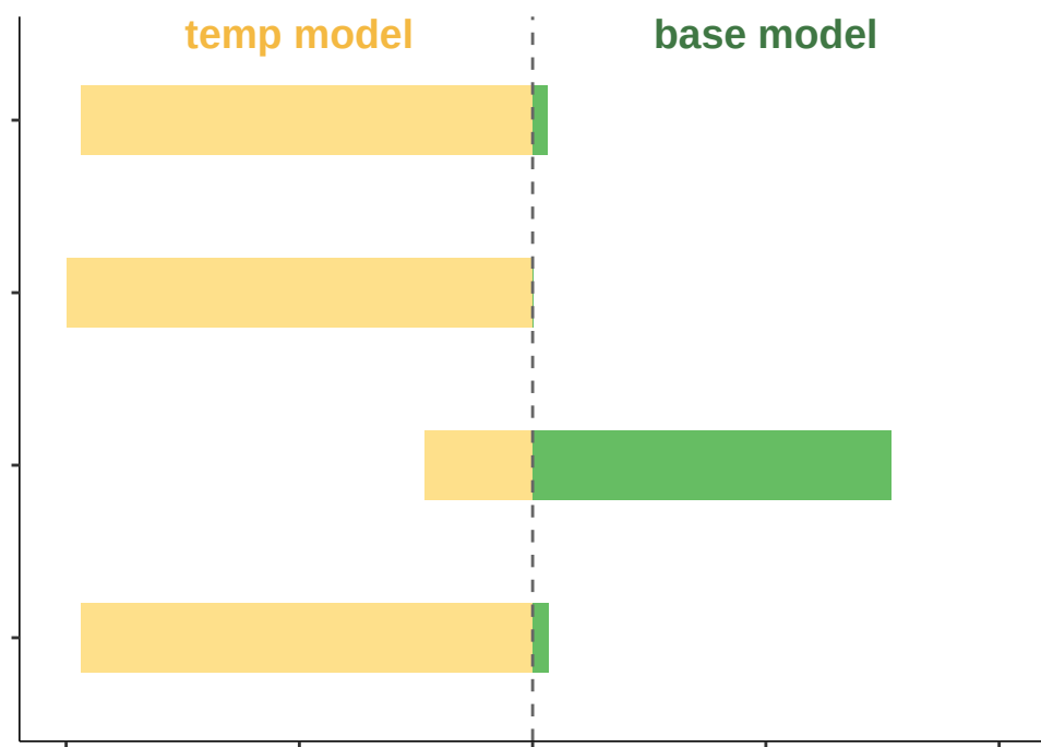
Metabolic pathway model weights
