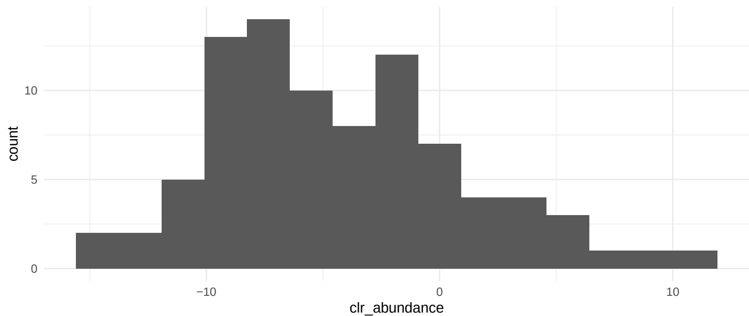
Distribution for 03258 Virion – Bacteriophage lambda
