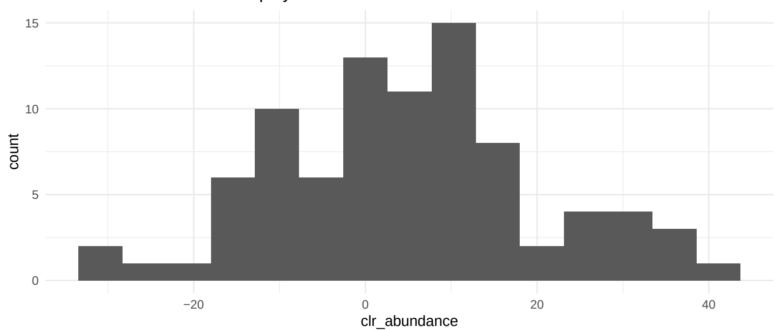
Distribution for 03020 RNA polymerase
