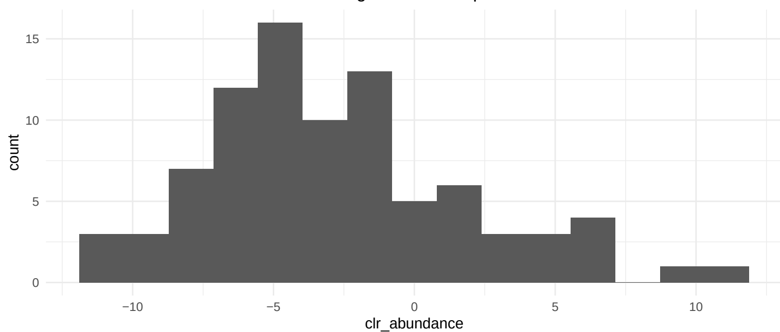
Distribution for 05208 Chemical carcinogenesis – reactive oxygen species
