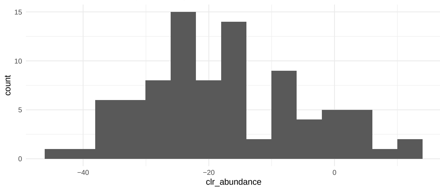
Distribution for 00330 Arginine and proline metabolism
