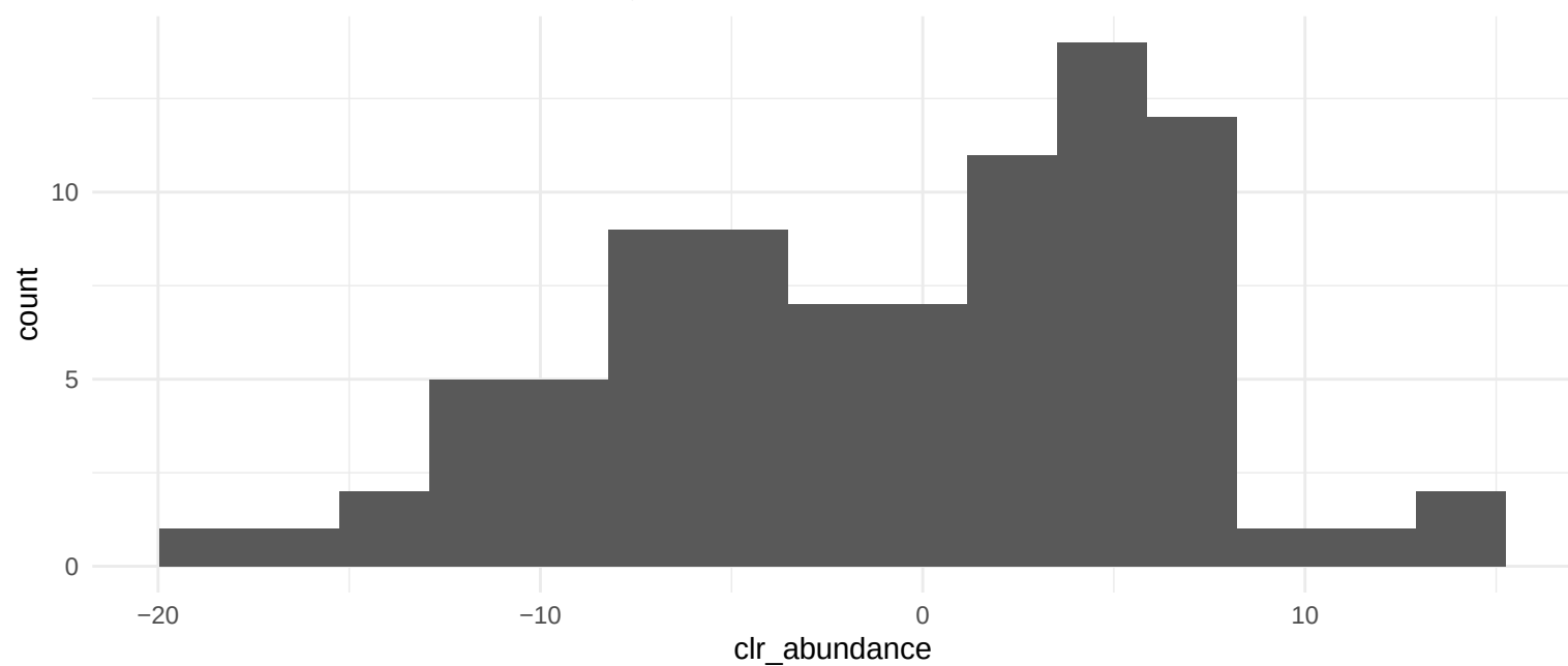
Distribution for 00830 Retinol metabolism
