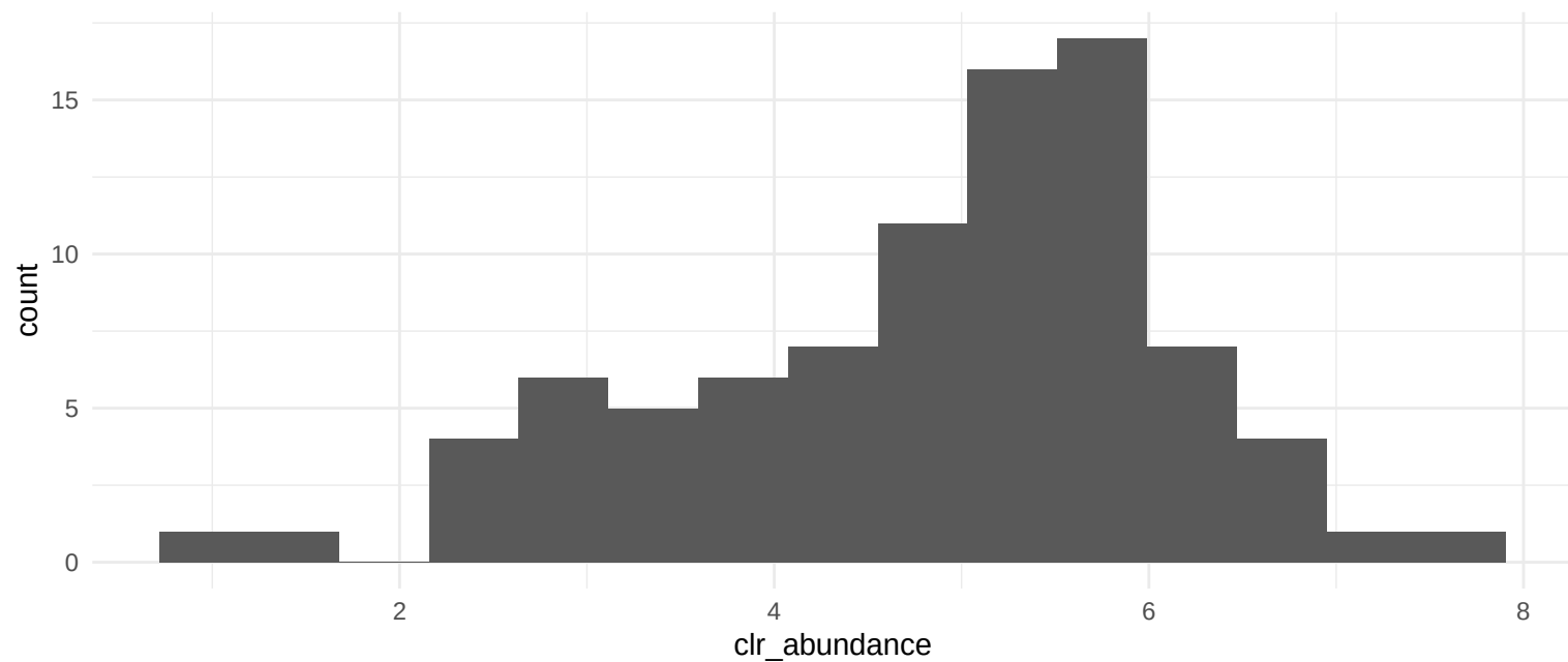
Distribution for 00999 Biosynthesis of various plant secondary metabolites
