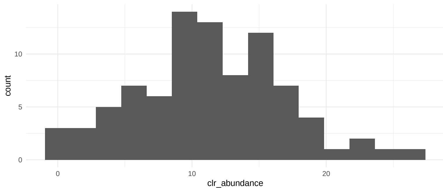
Distribution for 01007 Amino acid related enzymes
