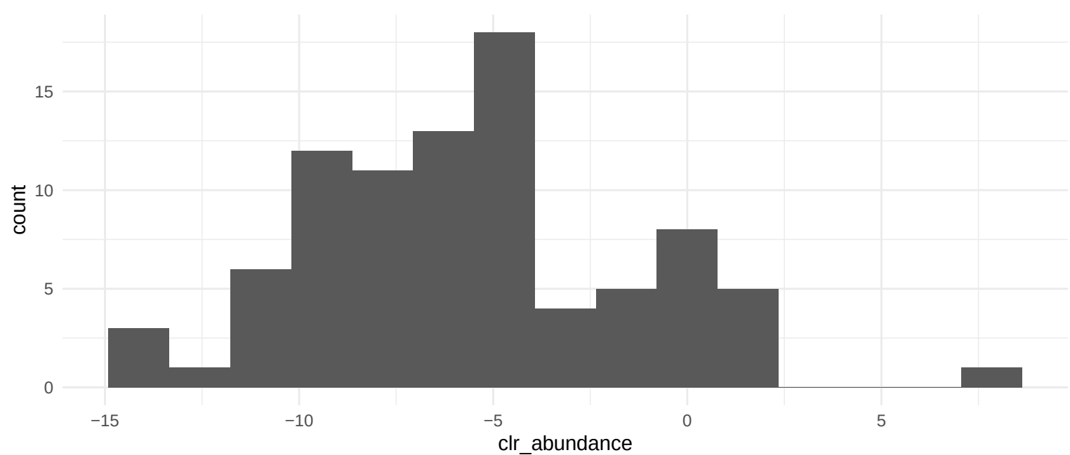
Distribution for 05215 Prostate cancer
