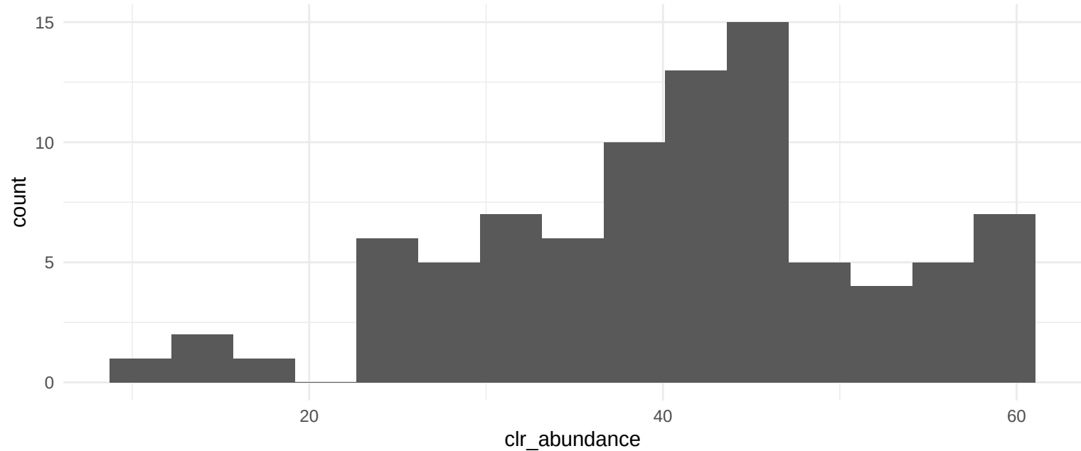
Distribution for 00062 Fatty acid elongation
