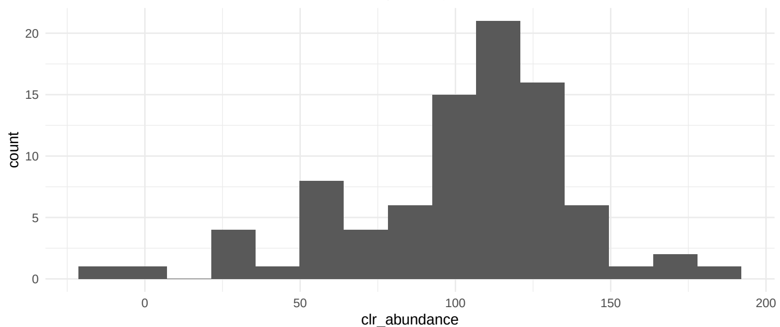
Distribution for 00730 Thiamine metabolism
