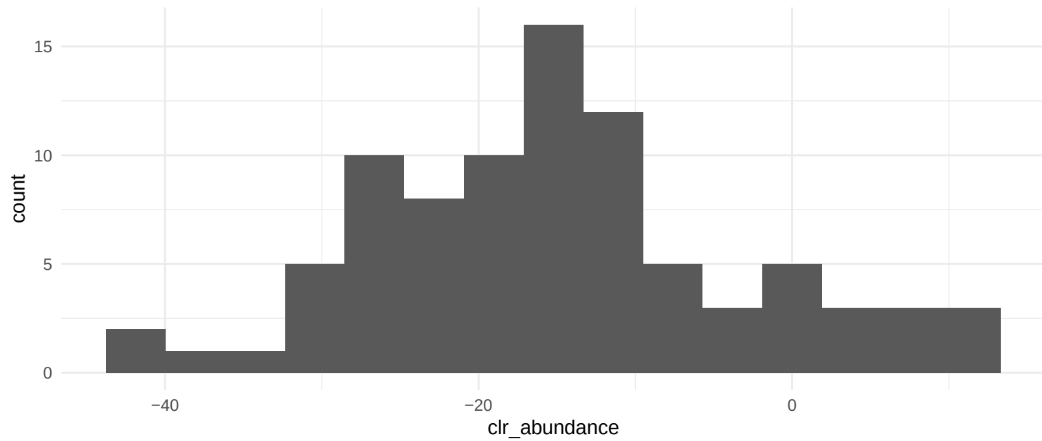
Distribution for 04111 Cell cycle – yeast
