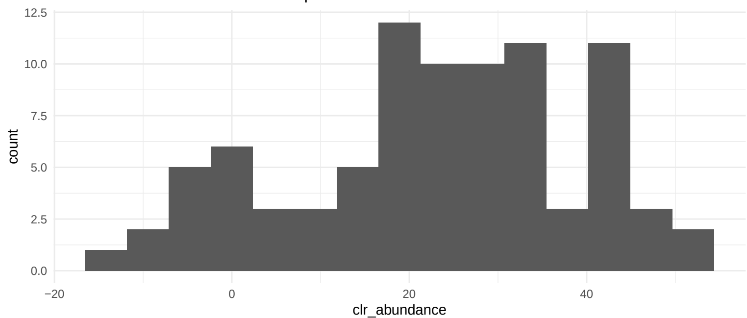
Distribution for 00460 Cyanoamino acid metabolism
