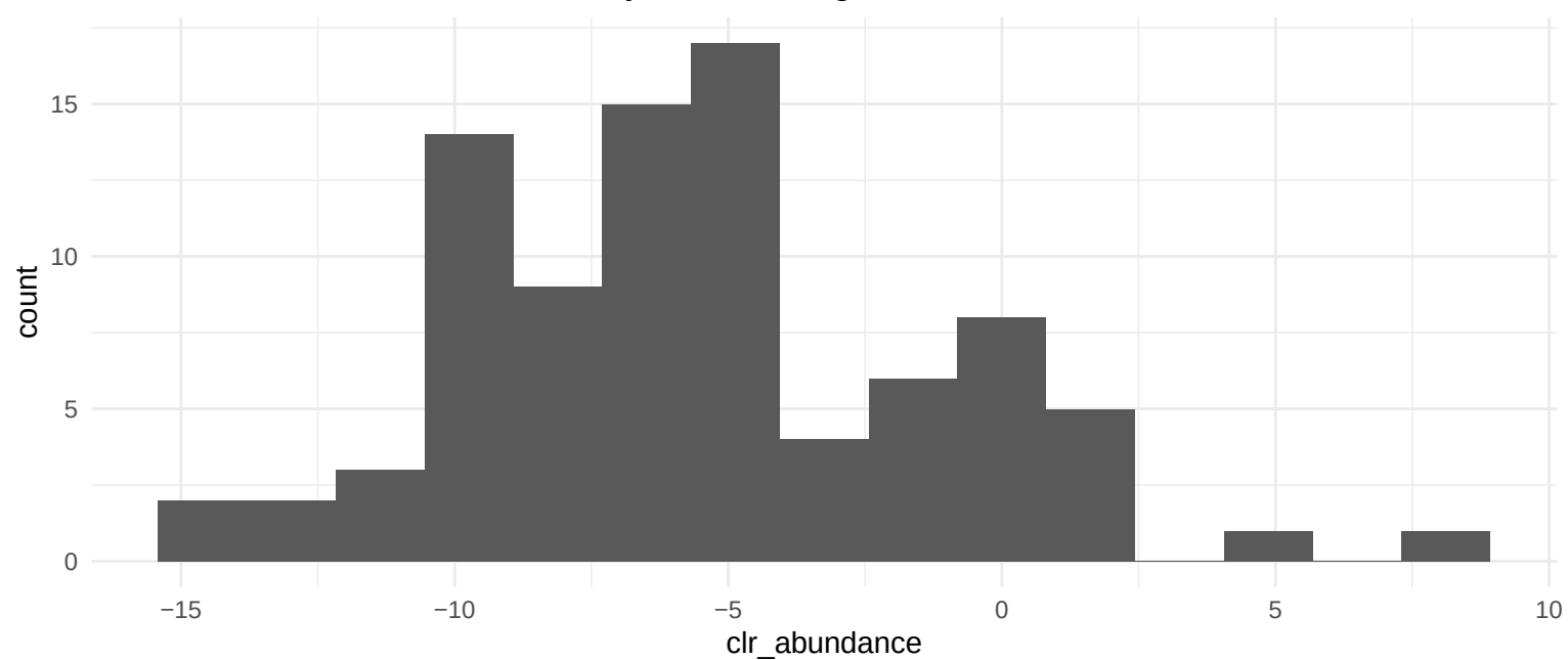
Distribution for 04810 Regulation of actin cytoskeleton
