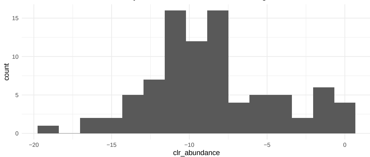
Distribution for 00361 Chlorocyclohexane and chlorobenzene degradation
