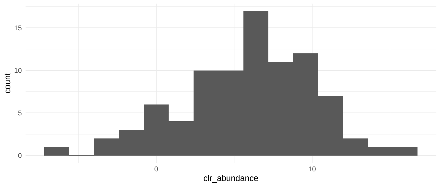
Distribution for 04070 Phosphatidylinositol signaling system
