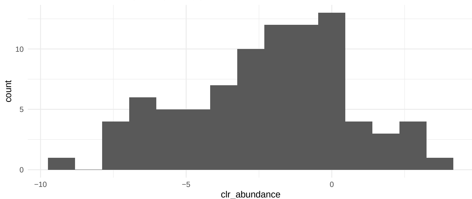
Distribution for 04120 Ubiquitin mediated proteolysis
