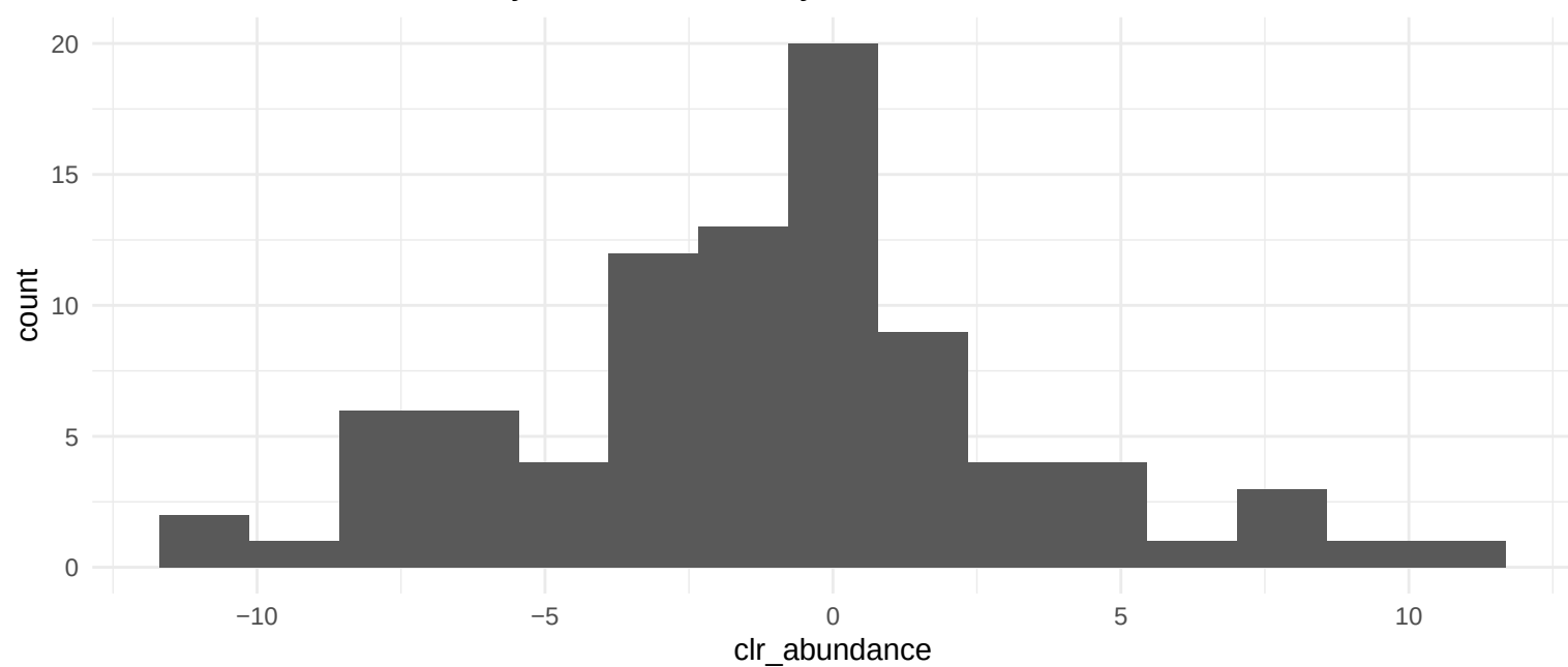
Distribution for 01052 Type I polyketide structures
