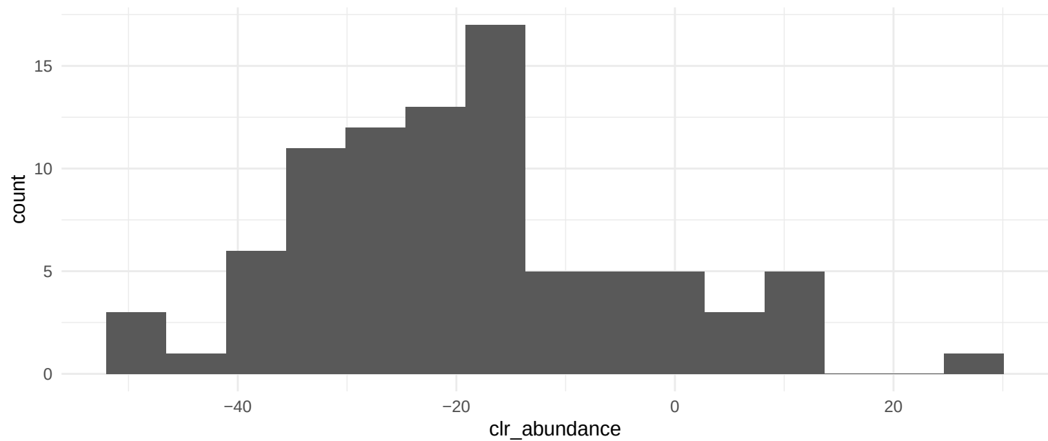
Distribution for 04114 Oocyte meiosis
