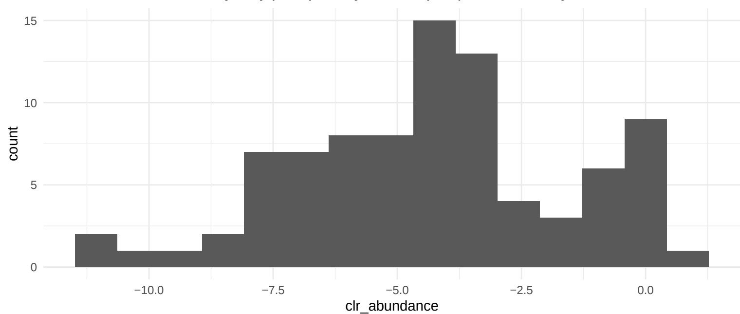
Distribution for 00564 Glycerophospholipid metabolism
