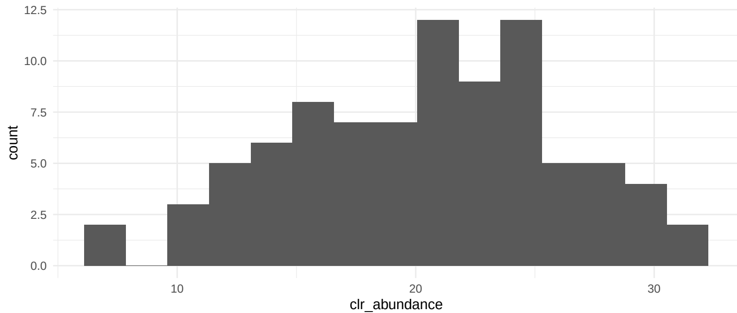
Distribution for 00660 C5-Branched dibasic acid metabolism
