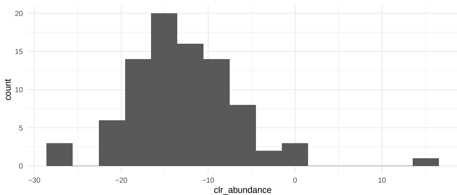
Distribution for 00430 Taurine and hypotaurine metabolism
