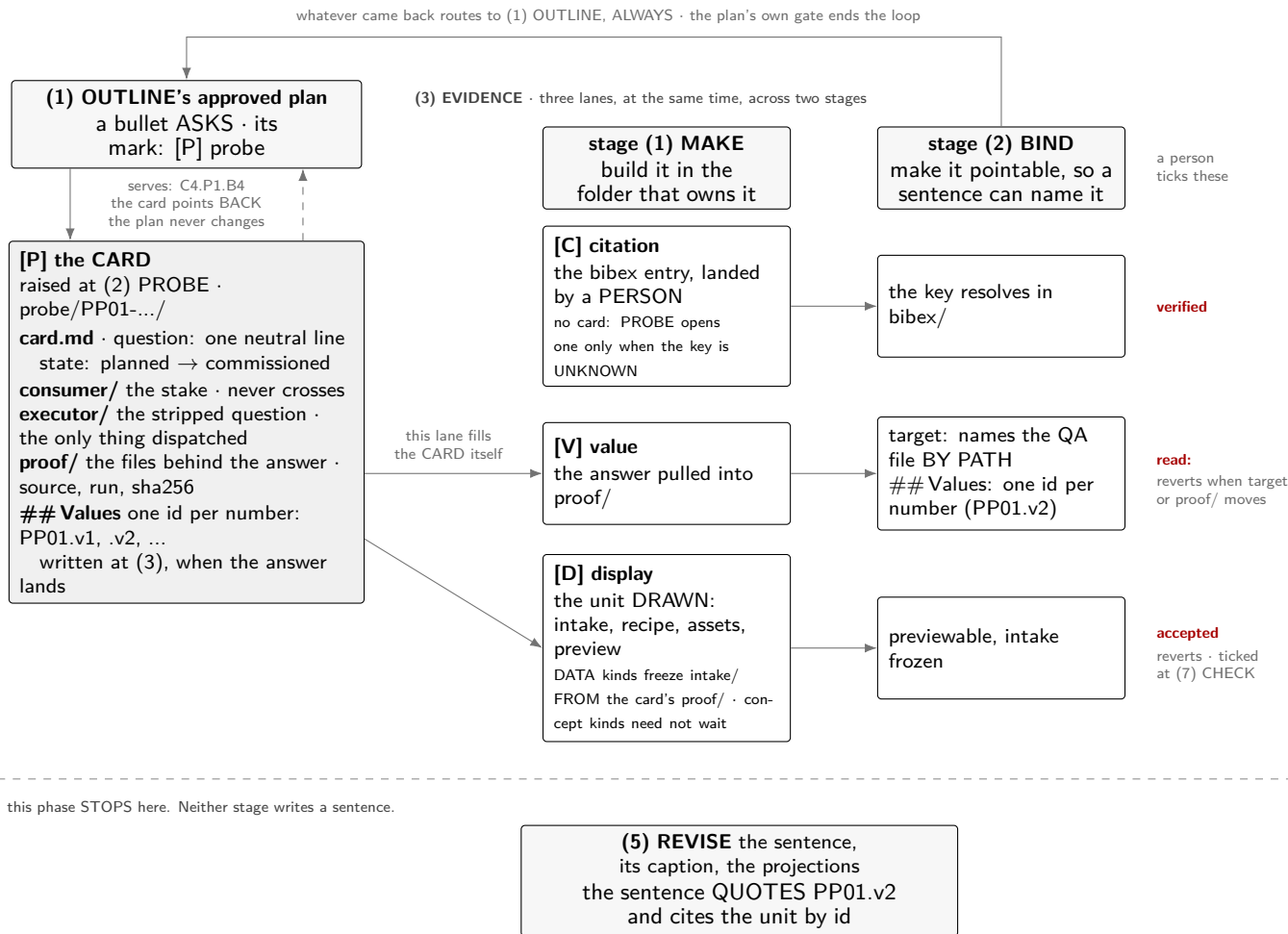
Figure 1: EVIDENCE, whole, with its head: the plan's bullet ASKS, PROBE raises the card (consumer/, executor/, proof/, and one id per value), and the three lanes run through MAKE and BIND at the same time. The value lane fills the card itself; a DATA display freezes its intake from the card's proof/; the citation lane is a person's and does not pass through the card. Two ticks revert; accepted is CHECK's. Neither stage writes a sentence; REVISE does, quoting one value by its id.
