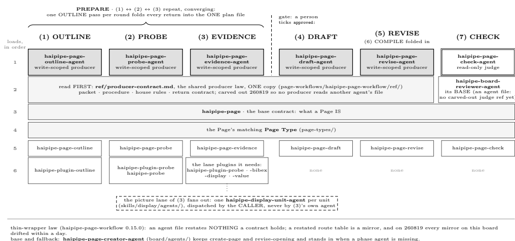
Figure 2: Who executes each phase, and what each loads: one agent per phase under page-workflows/agents/ (six files; (6) COMPILER is folded into (5), and (7)'s judge is haipipe-page-check-agent ), each walking one fixed stack whose shared law lives once in ref/producer-contract.md . The PREPARE trio (1)(2)(3) repeats until the plan converges and stops at a person's approved: tick. The full routes and stop conditions are Display4's and Display1's.
