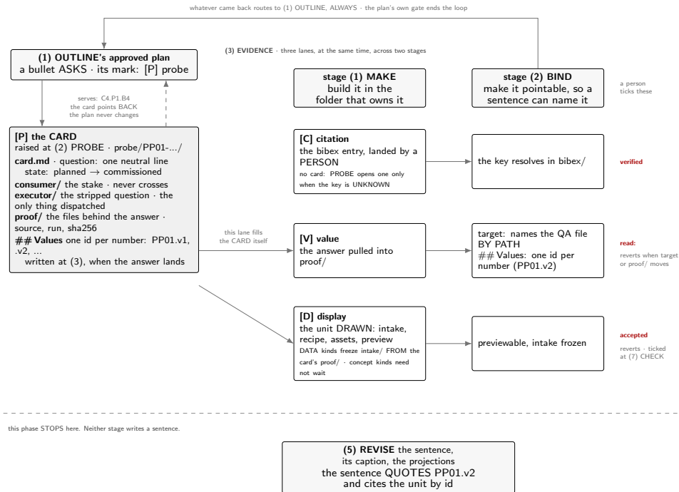
Figure 3: EVIDENCE, whole, with its head: the plan's bullet ASKS, PROBE raises the card (consumer/, executor/, proof/, and one id per value), and the three lanes run through MAKE and BIND at the same time. The value lane fills the card itself; a DATA display freezes its intake from the card's proof/; the citation lane is a person's and does not pass through the card. Two ticks revert; accepted is CHECK's. Neither stage writes a sentence; REVISE does, quoting one value by its id.
