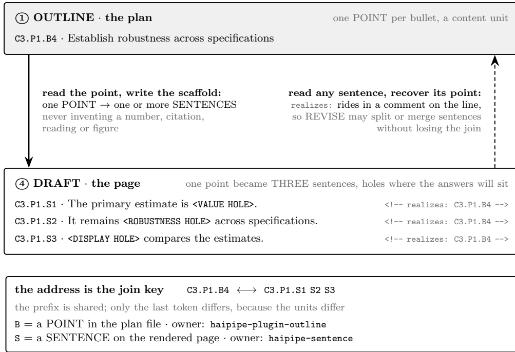
Figure 5: The point-to-sentence conversion at ④ DRAFT, shown both ways round. Forward: one approved outline POINT (C3.P1.B4) becomes one or more sentence scaffolds (C3.P1.S1–S3), each hole sitting exactly where its answer will sit, and DRAFT may never invent the value, citation, reading or figure. Backward: the machine-readable realizes: comment on each scaffold line recovers the point from any sentence, so REVISE can split or merge sentences without losing the join. The shared C3.P1 prefix is the join key; B (a point in the plan) is owned by haipipe-plugin-outline, S (a sentence on the page) by haipipe-sentence, and neither redefines the other.
