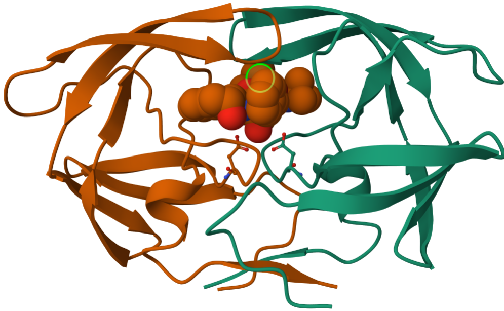
Figure 1: HIV Protease
