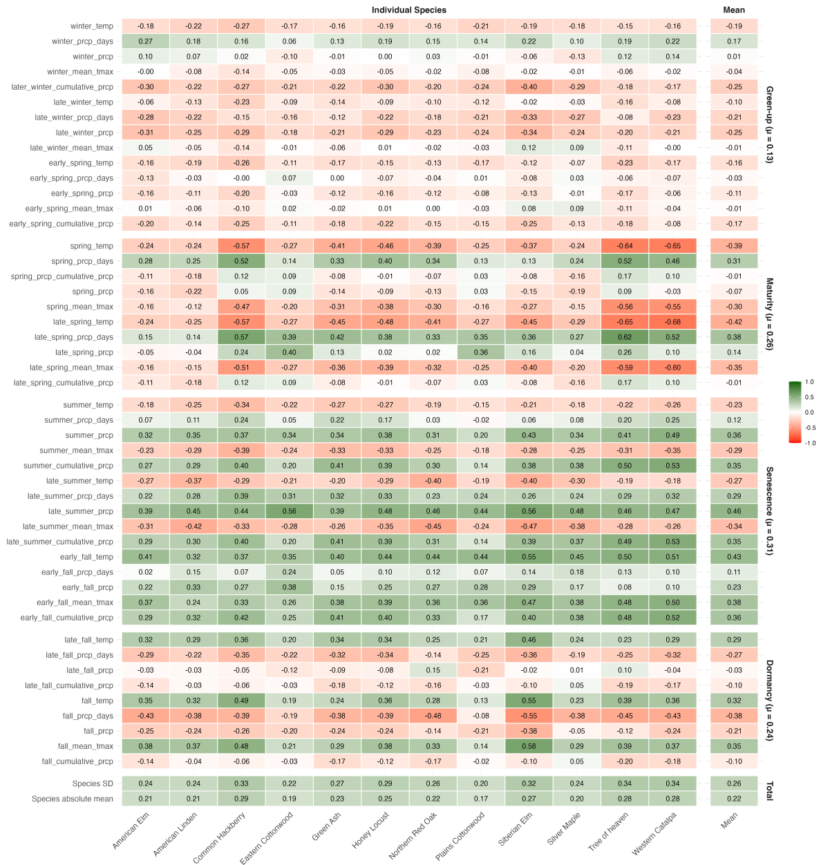
Figure 2: Pearson correlation coefficients between phenological timing and seasonal climate variables across 12 tree species. Correlations are shown for individual species and the cross-species average. Green indicates positive correlations (later phenology with higher values), red indicates negative correlations (earlier phenology with higher values). Climate variables were selected based on biological relevance to each phenological stage (see Table 2 for seasonal definitions).
