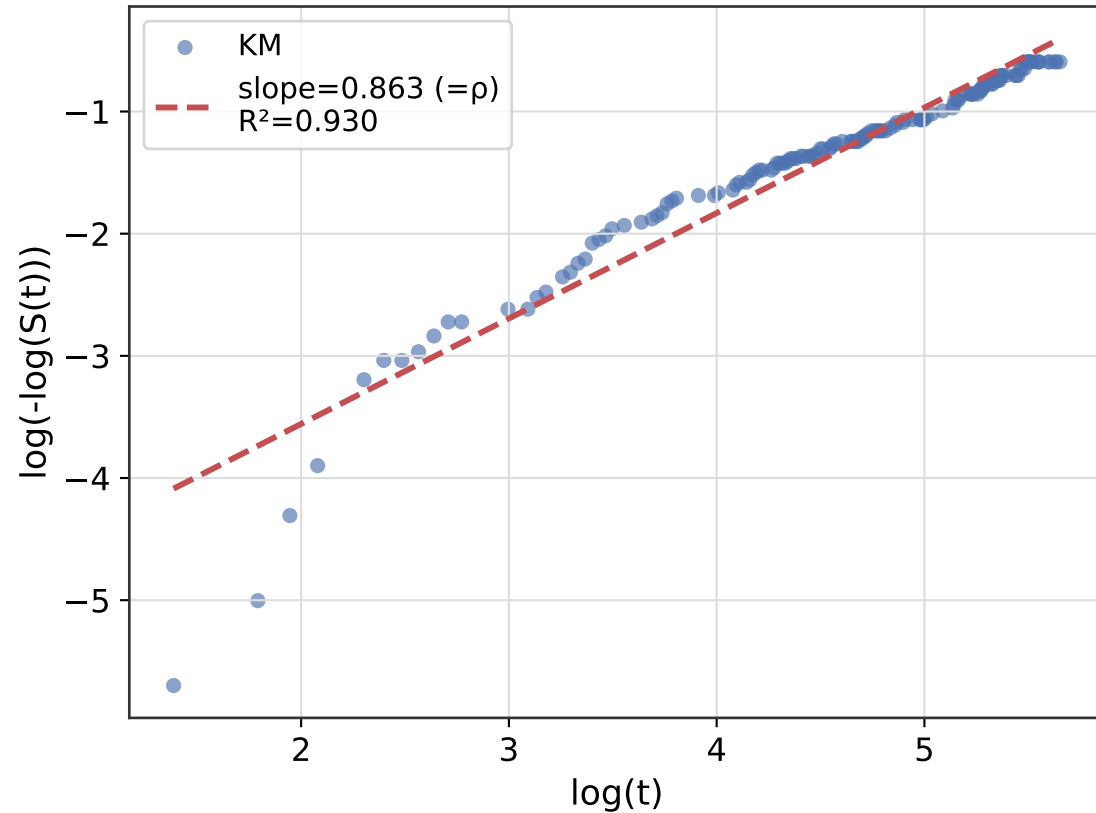
Weibull Probability Plot
