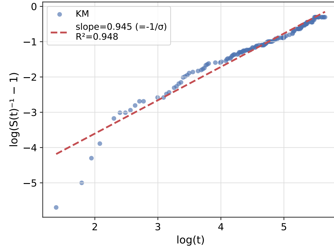
Log-Logistic Probability Plot
