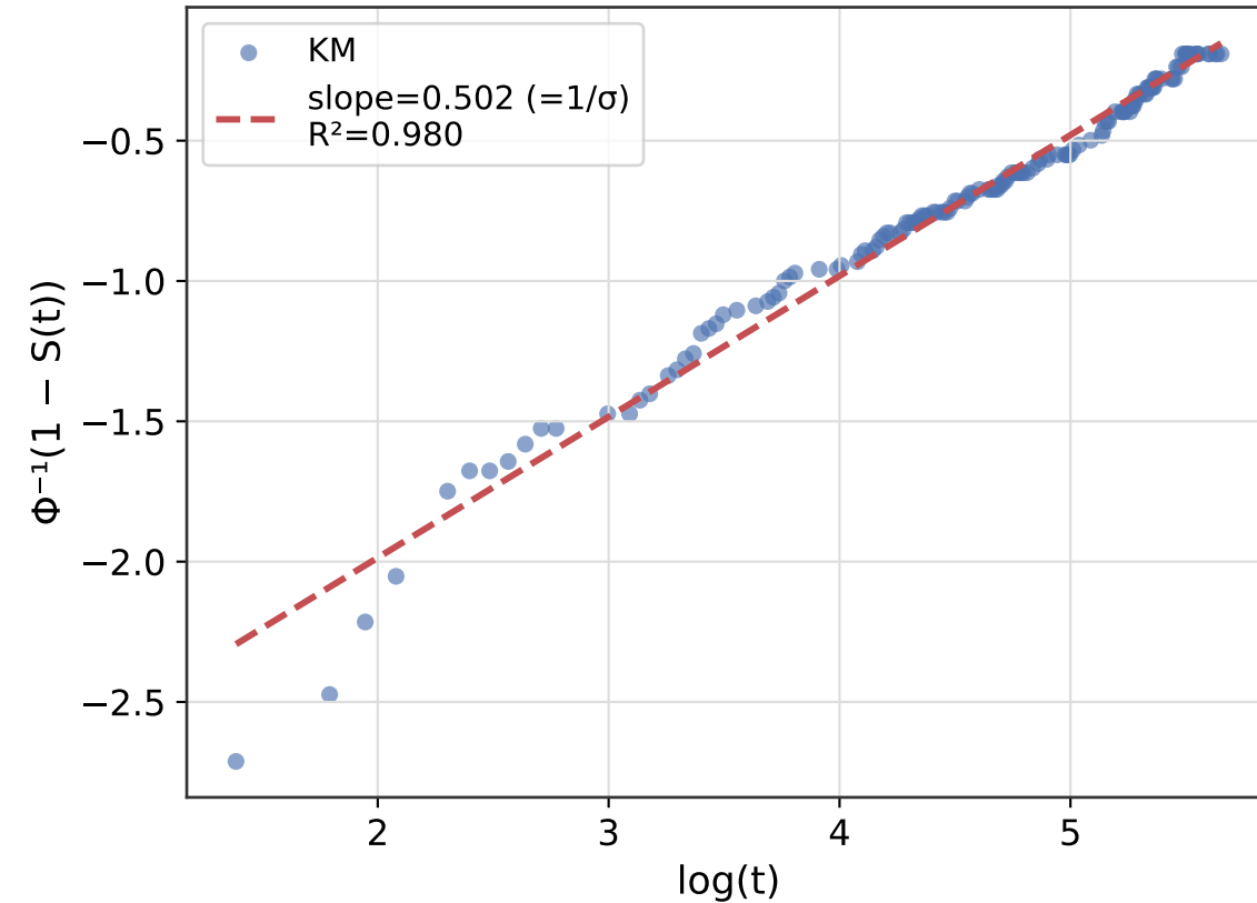
Log-Normal Probability Plot
