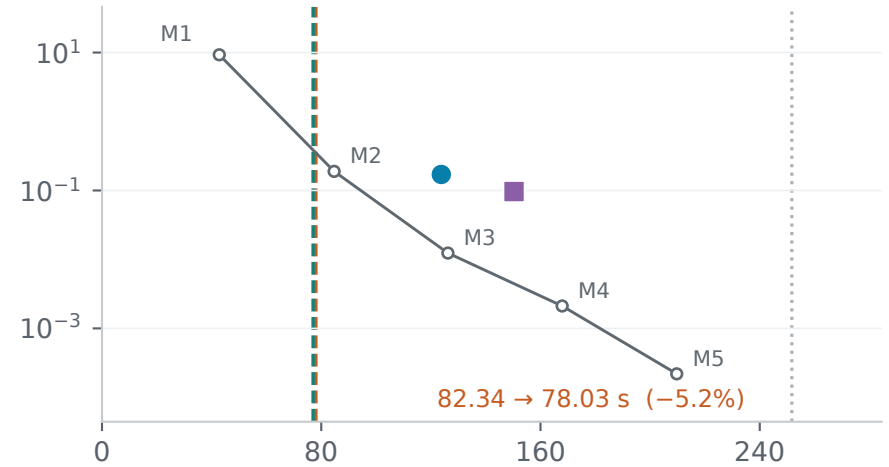
Tanaka
