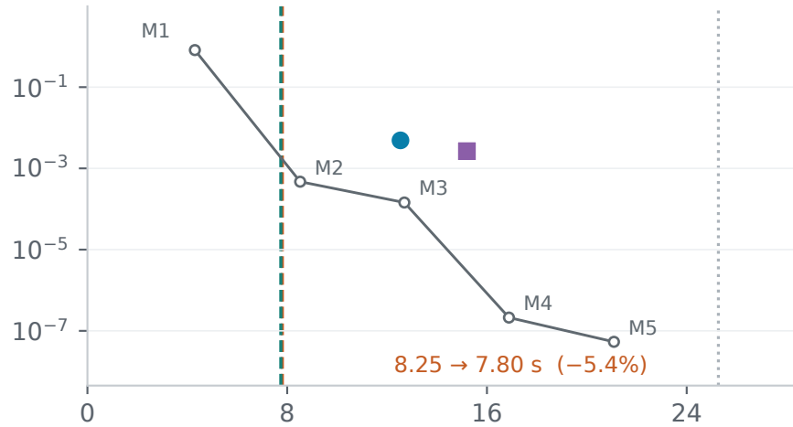
Stokes
