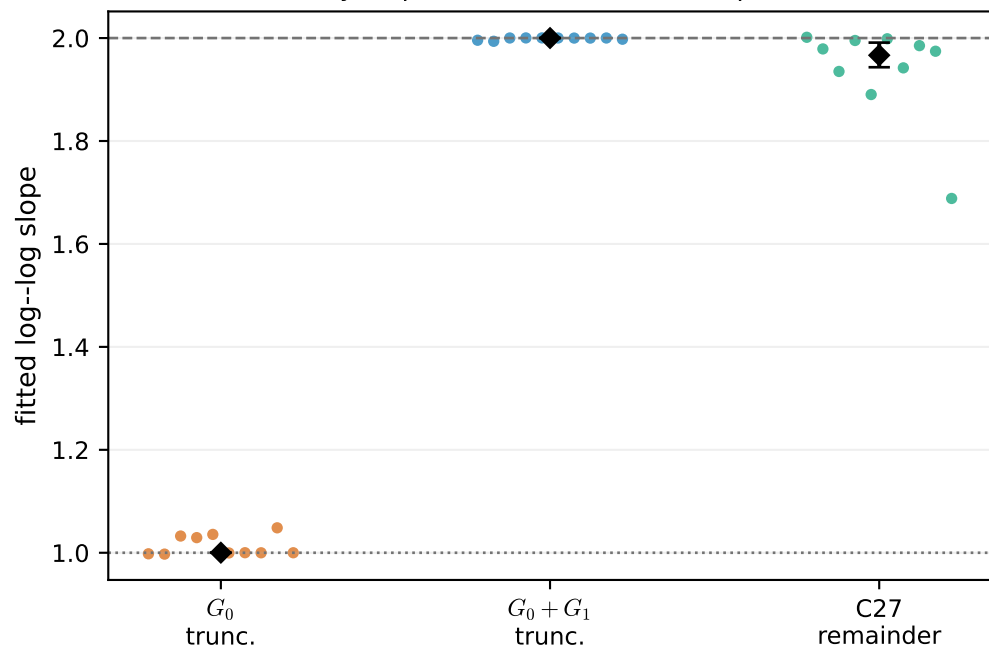
(b) Family slopes; black diamonds are pooled fits
