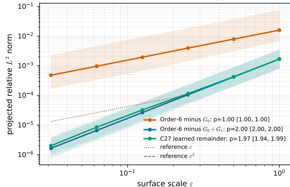
(a) Small-amplitude convergence, |k| \leq 128
