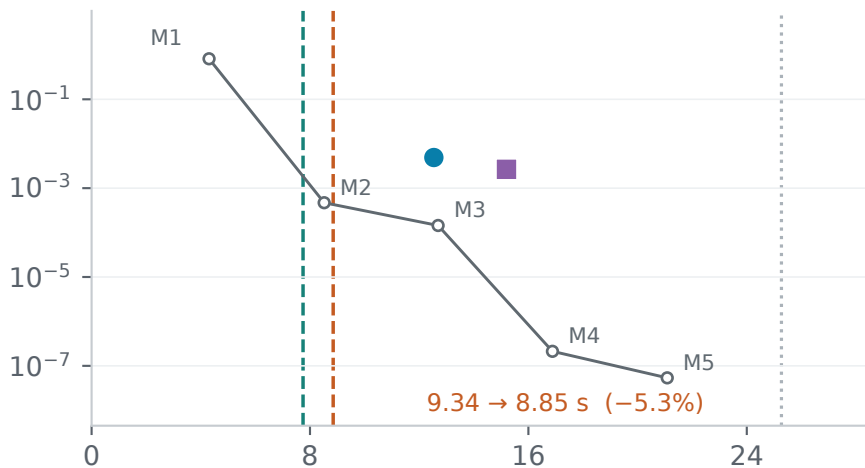
Stokes
