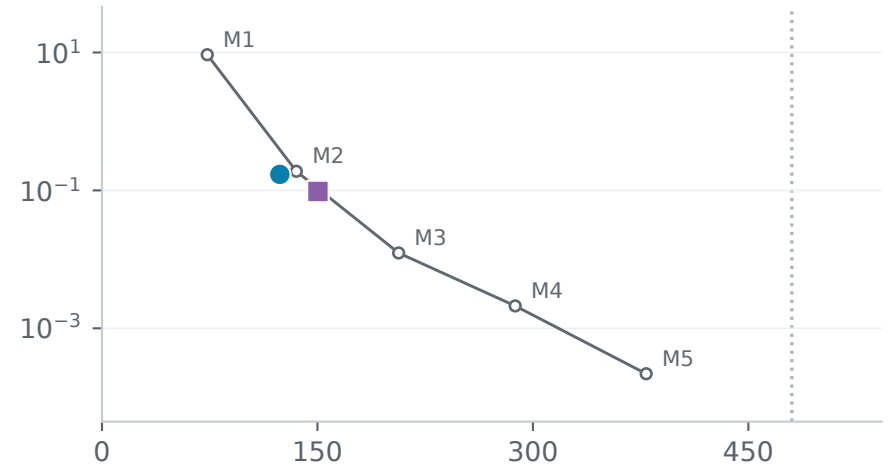
Tanaka
