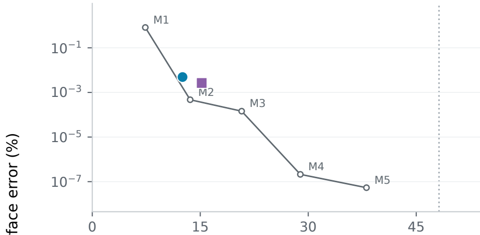
Stokes
