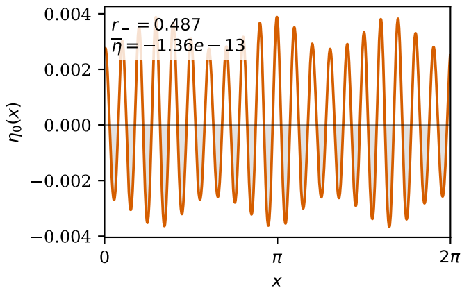
(c) Benjamin-Feir, case 11: guard inactive
