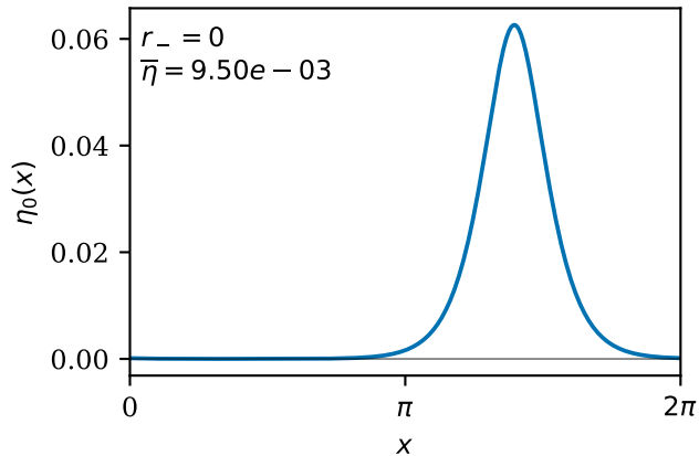
(c) Benjamin-Feir, case 11: guard inactive
