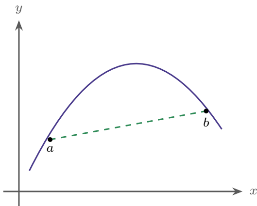
Concave
