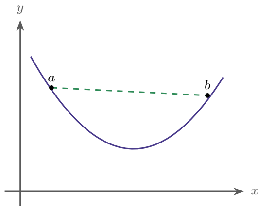
Convexe
