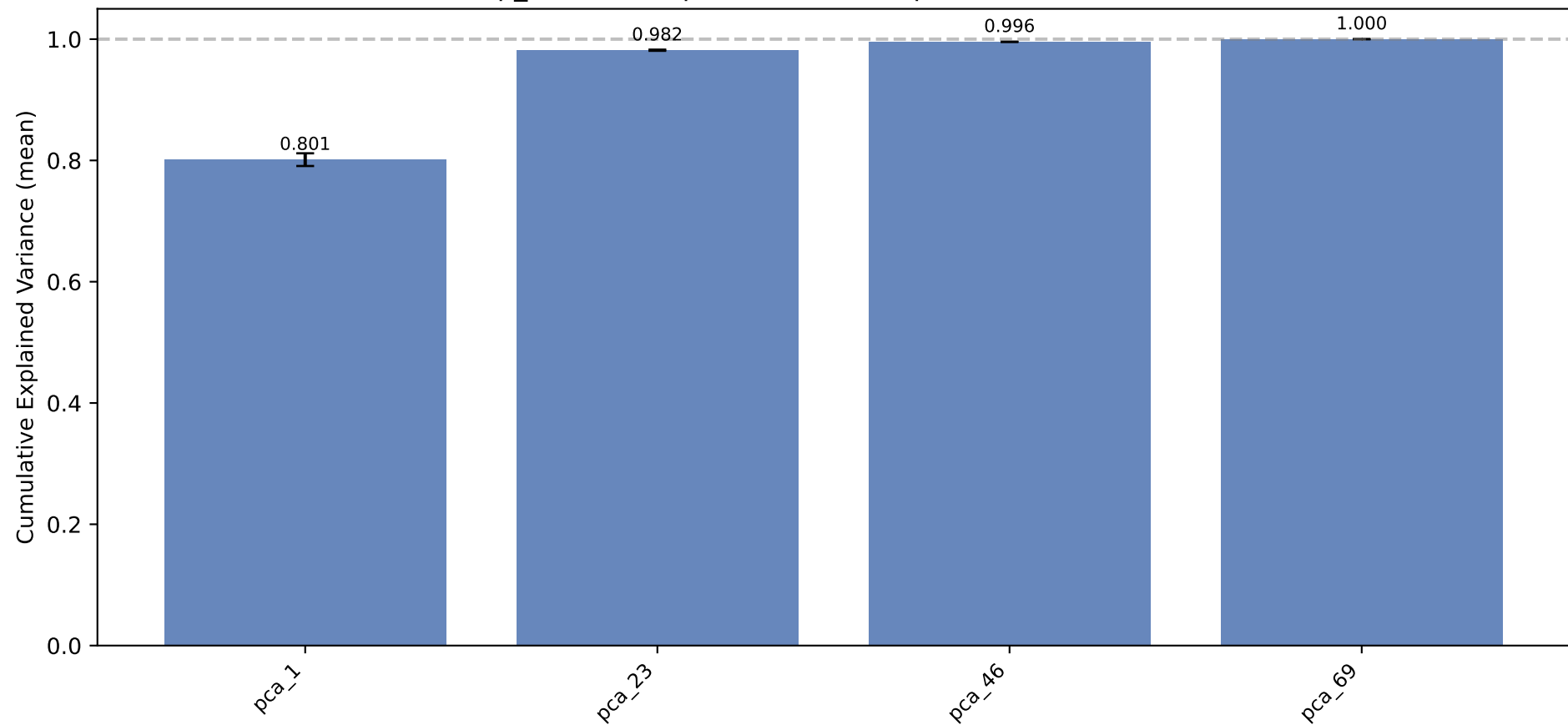
exp_9 — PCA Explained Variance per Condition (MCCV)
