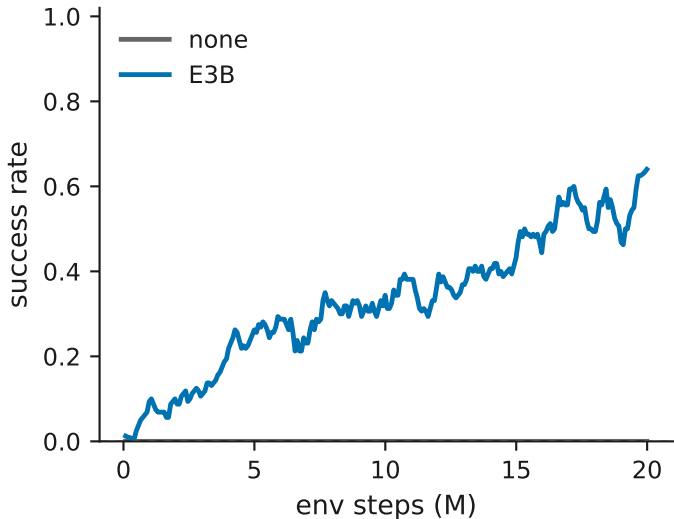
MysteryPath penalty (GatedDeltaNet)
