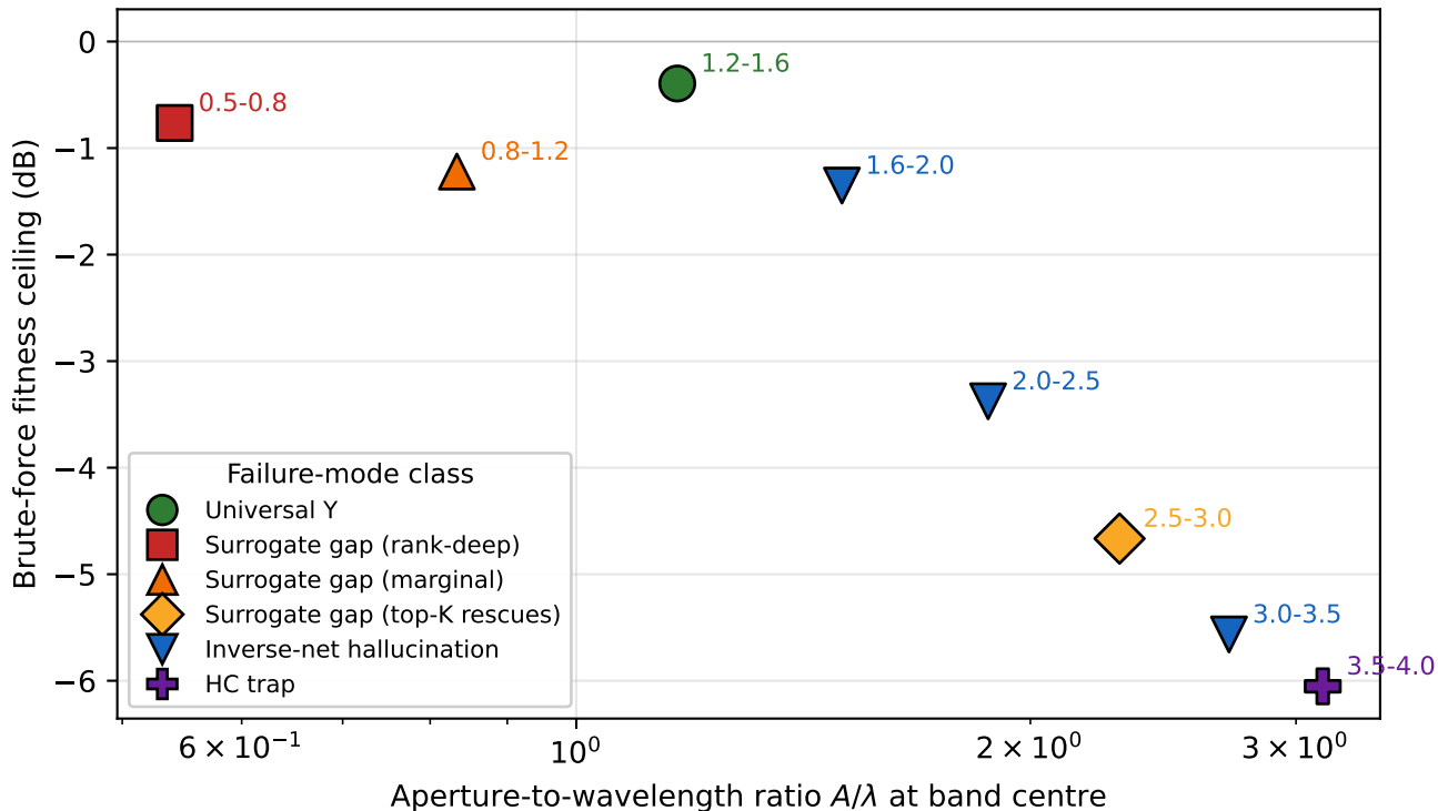
24-bit BF fitness ceiling vs aperture electrical size, coloured by failure-mode class ( \backslash S \sim 6 )
