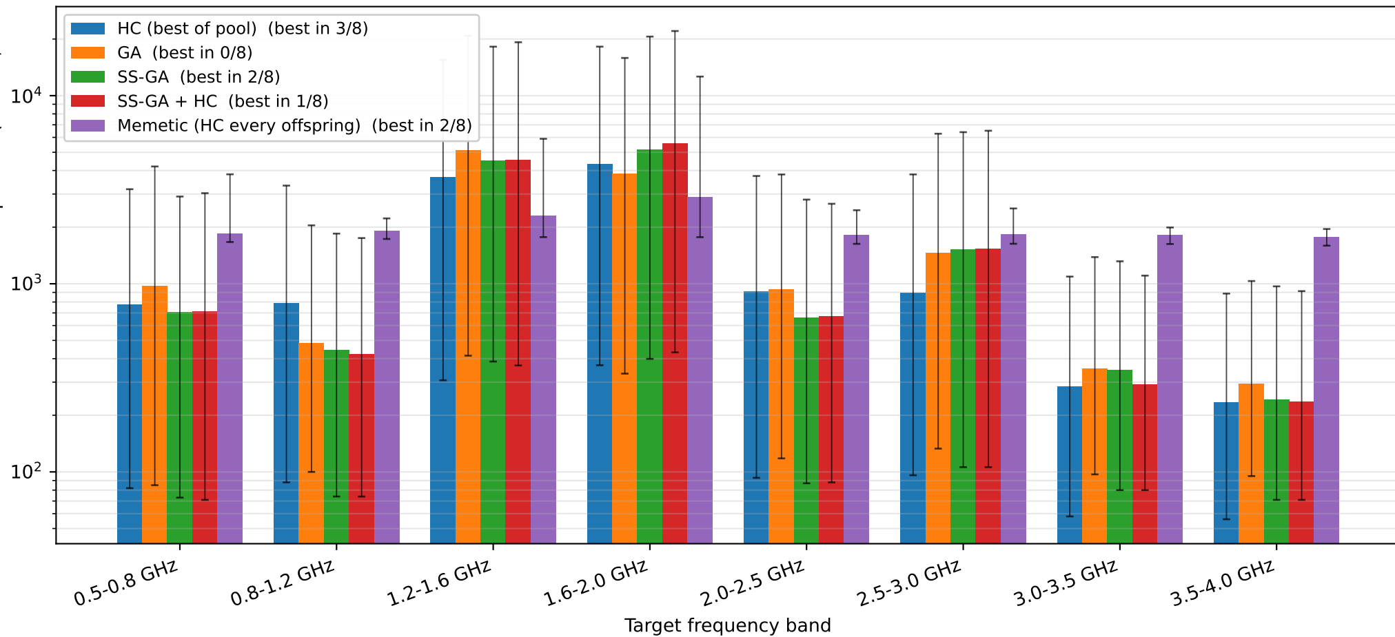
20-bit fragmented aperture: optimizer comparison across 8 bands ( 2^{20} exhaustive ground truth; 1 000 trials per method per band)
