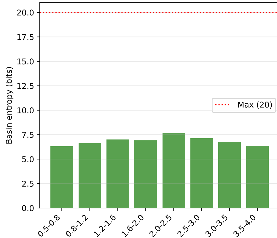
Basin Entropy per Band
