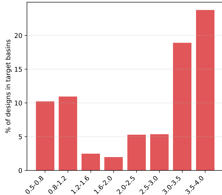
Target Basin Coverage per Band
