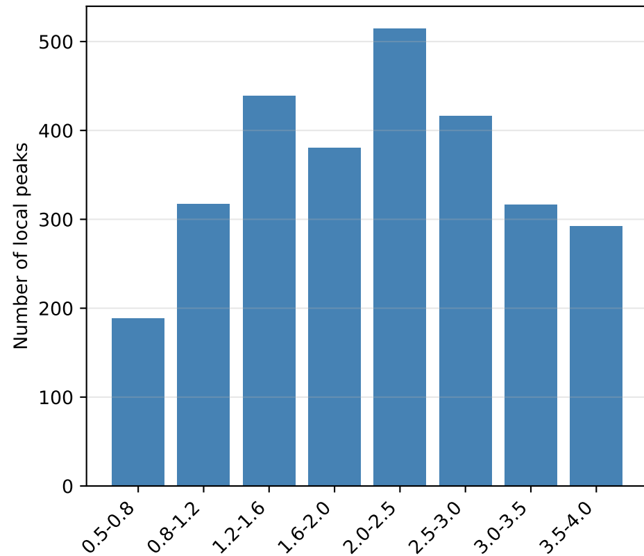
Distinct Peaks per Band
