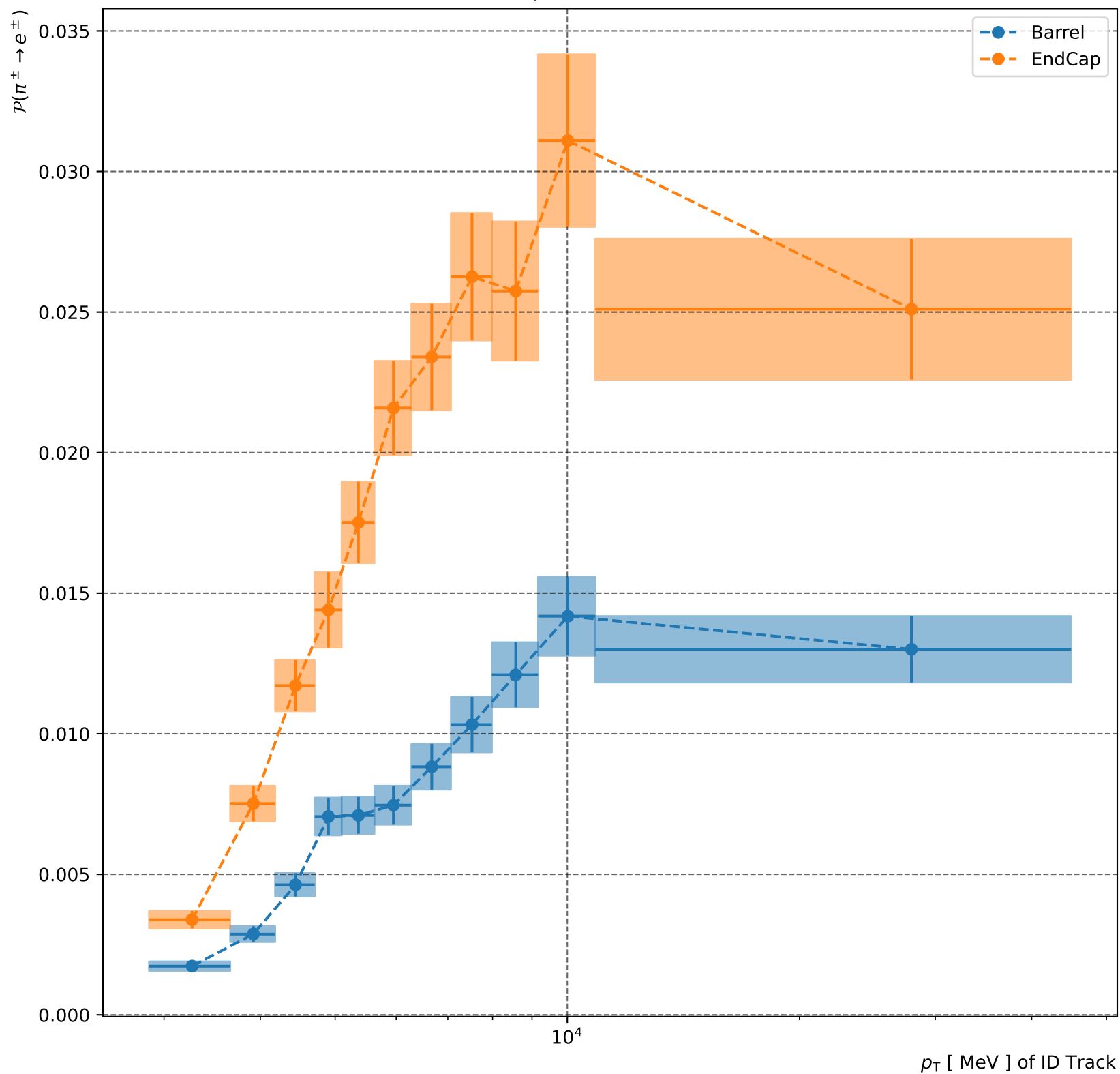
Electron Fake Rate w/ B^0 \rightarrow K^* e^+ e^- at LH: LHVeryLooseNod0. Binned to Cap Statistical Error at 10.0%
