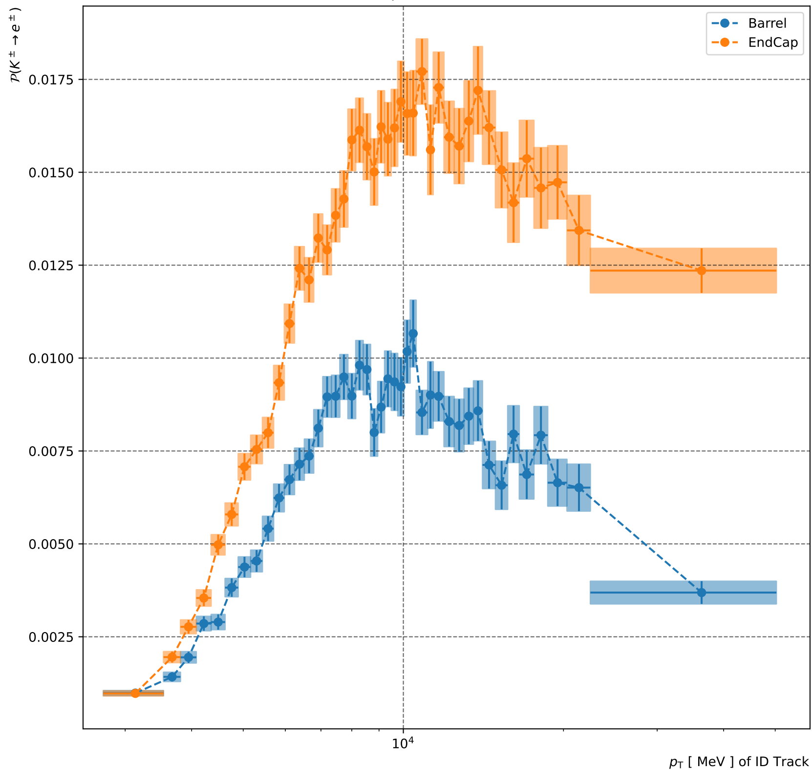
Electron Fake Rate w/ B^+ \rightarrow J/\psi(\rightarrow \mu^+ \mu^-)K^+ at LH: LHVeryLooseNod0. Binned to Cap Statistical Error at 10.0%
