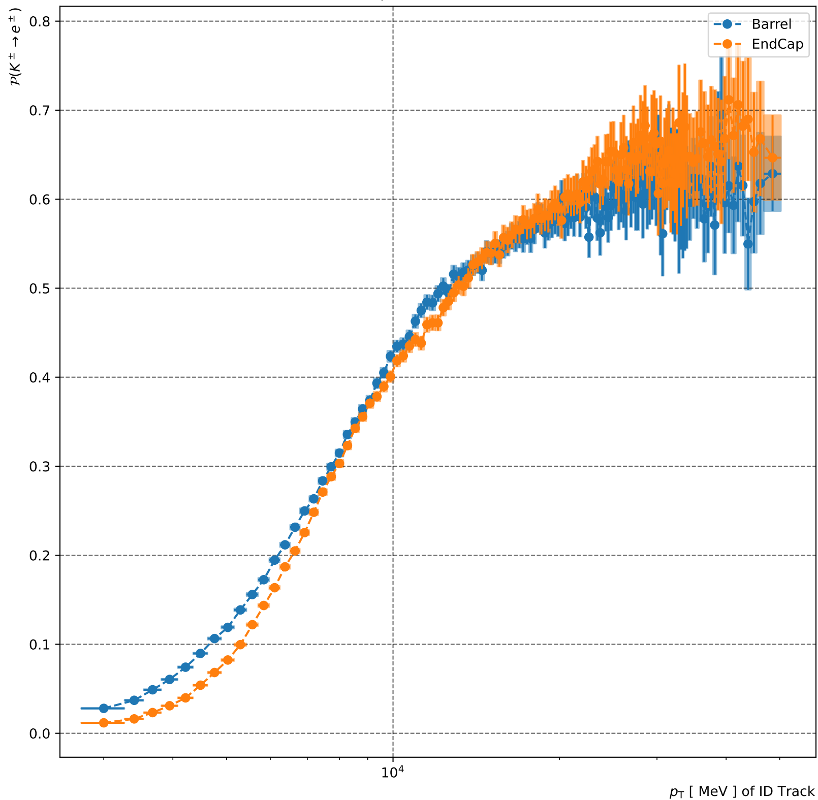
Electron Fake Rate w/ B^+ \rightarrow J/\psi(\rightarrow \mu^+ \mu^-)K^+ at LH: None. Binned to Cap Statistical Error at 10.0%
