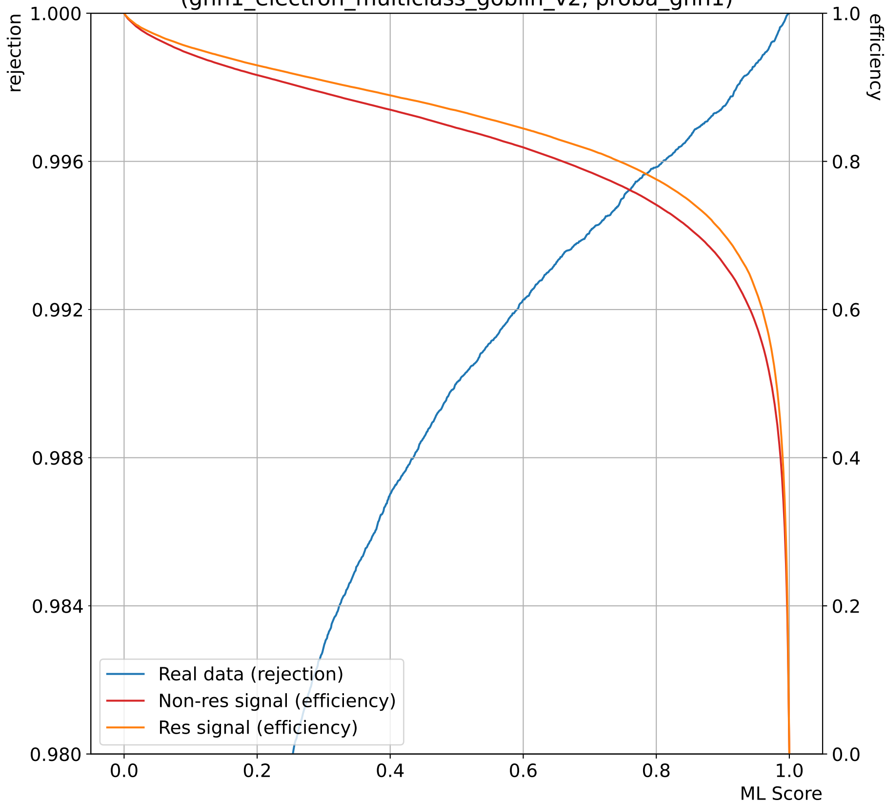
Efficiency in USR/rejection in NN1TRB, high q^2 (gnn1_electron_multiclass_goblin_v2, proba_gnn1)
