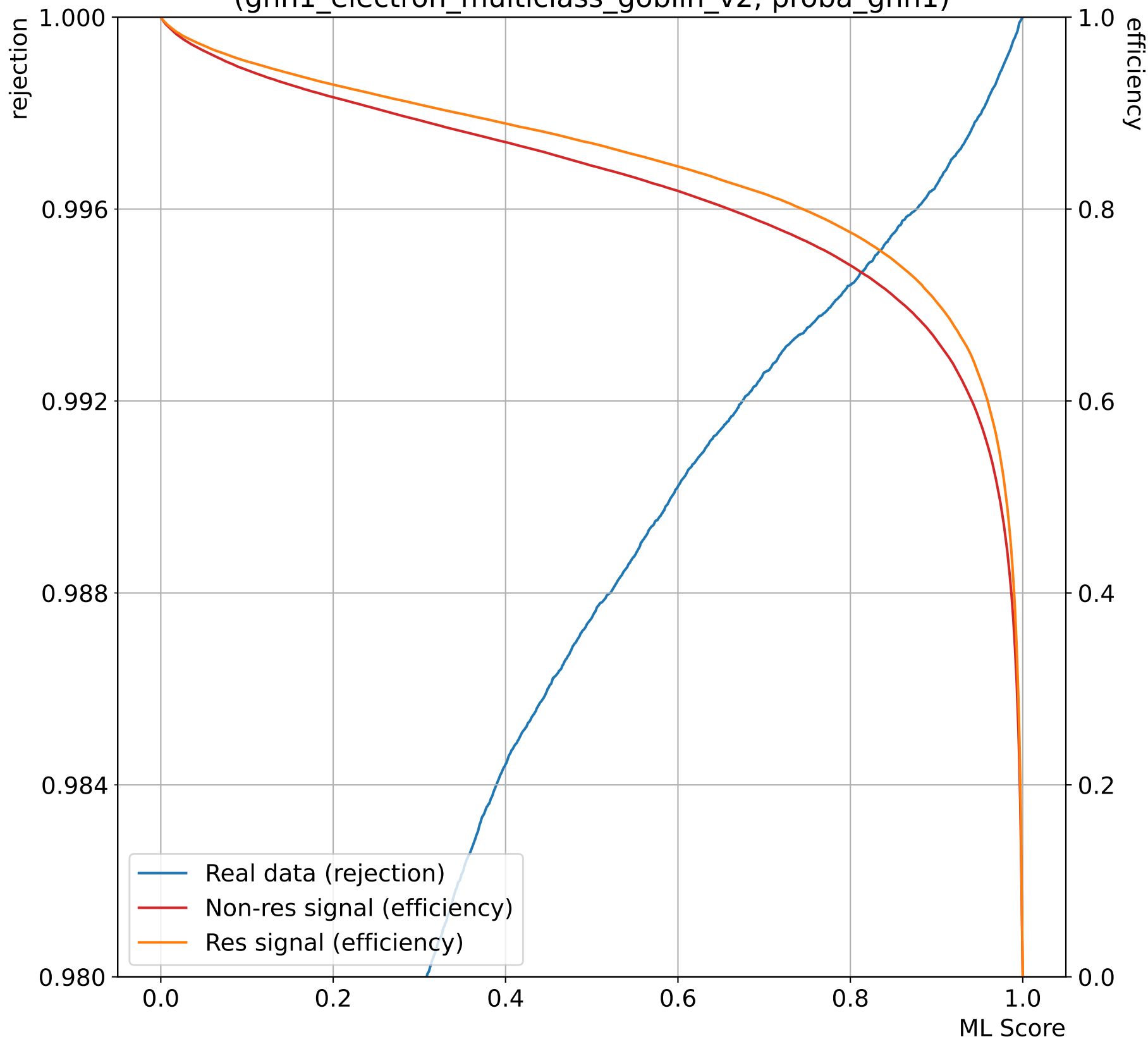
Efficiency in USR/rejection in NN2TRB, high q^2 (gnn1_electron_multiclass_goblin_v2, proba_gnn1)
