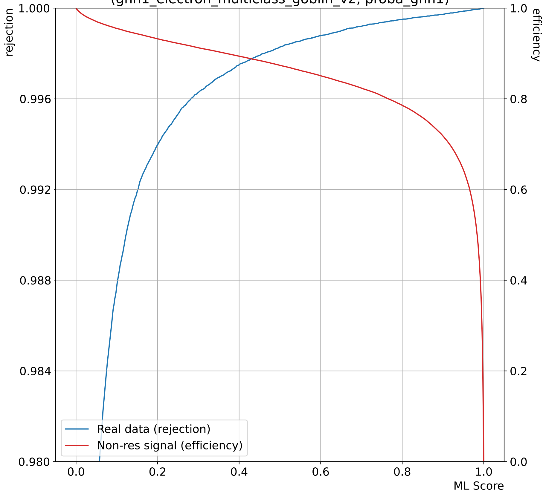
Efficiency in USR/rejection in NN2TRB, low q^2 (gnn1_electron_multiclass_goblin_v2, proba_gnn1)
