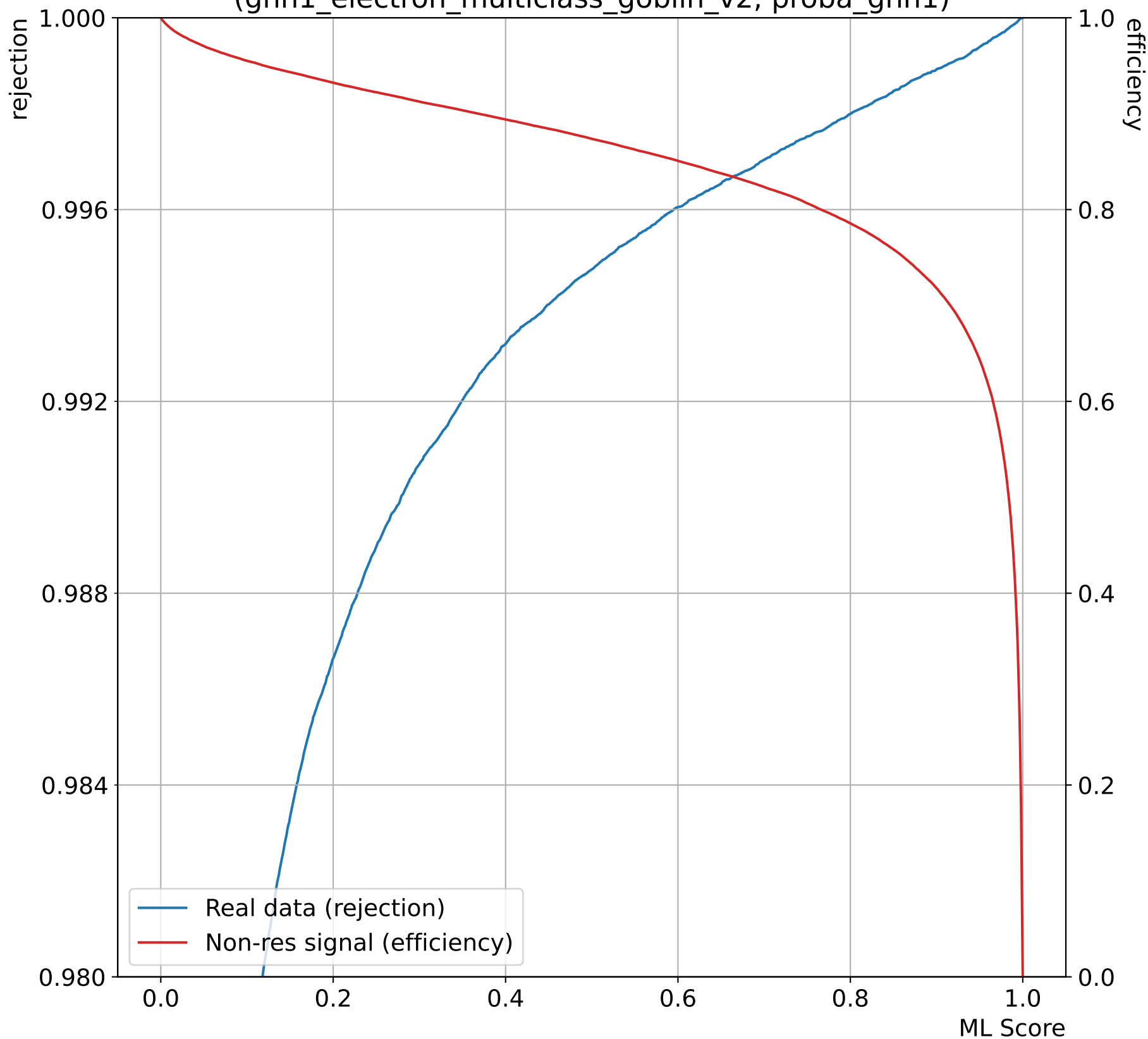
Efficiency in USR/rejection in NN1TRB, low q^2 (gnn1_electron_multiclass_goblin_v2, proba_gnn1)
