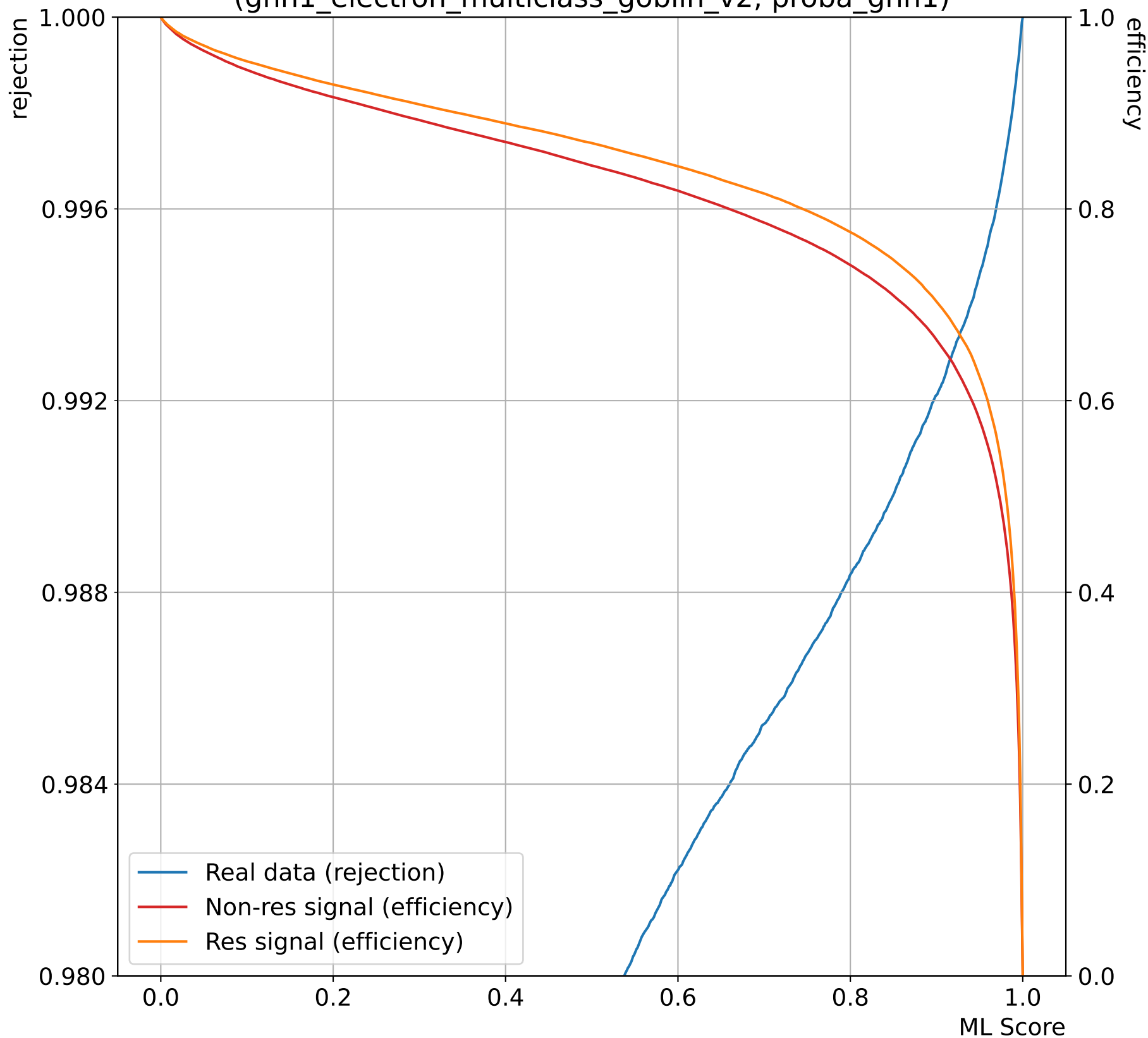
Efficiency/rejection in USR, high q^2 (gnn1_electron_multiclass_goblin_v2, proba_gnn1)
