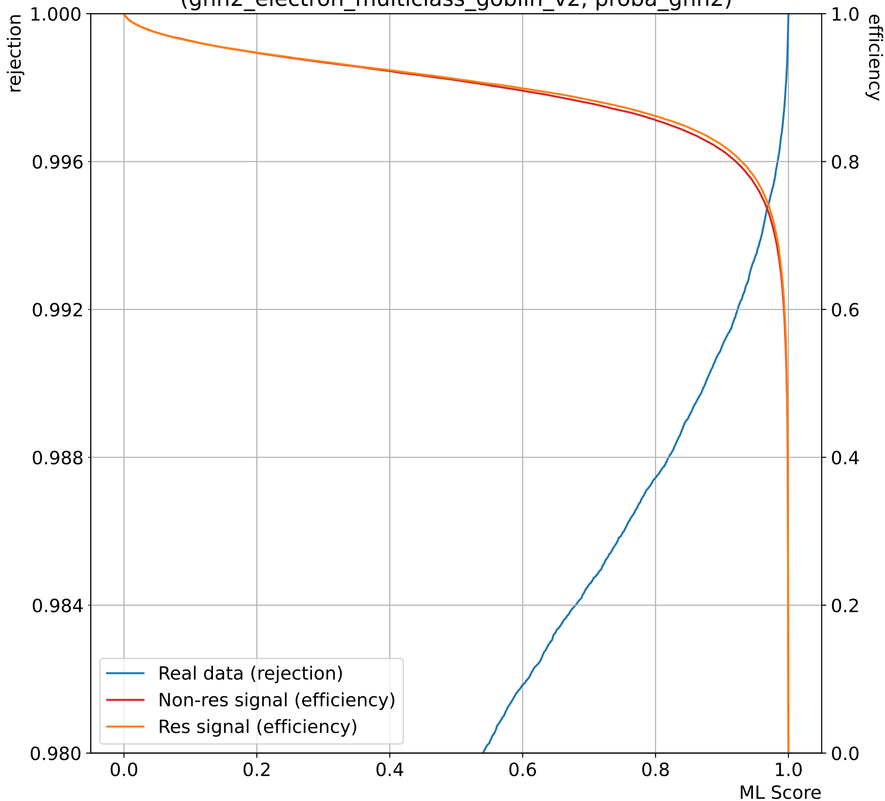
Efficiency in USR/rejection in NN2TRB, high q^2 (gnn2_electron_multiclass_goblin_v2, proba_gnn2)
