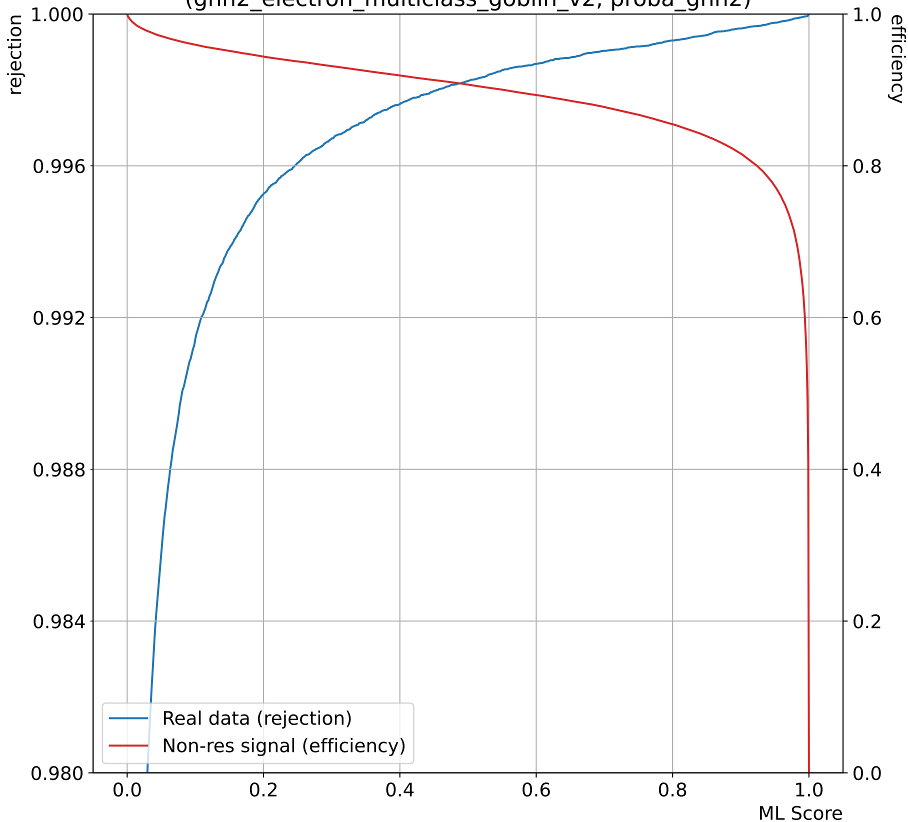
Efficiency in USR/rejection in NN2TRB, low q^2 (gnn2_electron_multiclass_goblin_v2, proba_gnn2)
