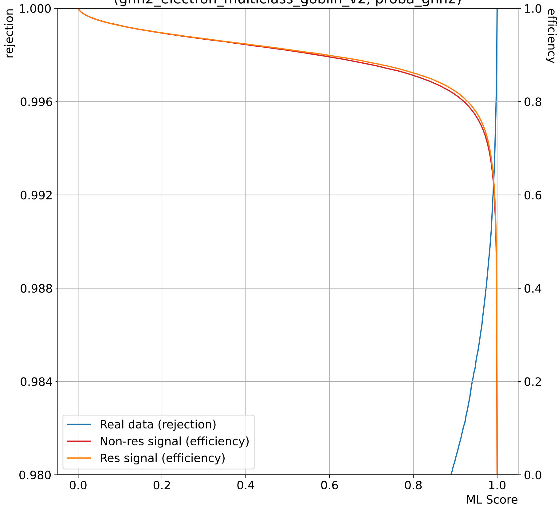
Efficiency/rejection in USR, high q^2 (gnn2_electron_multiclass_goblin_v2, proba_gnn2)
