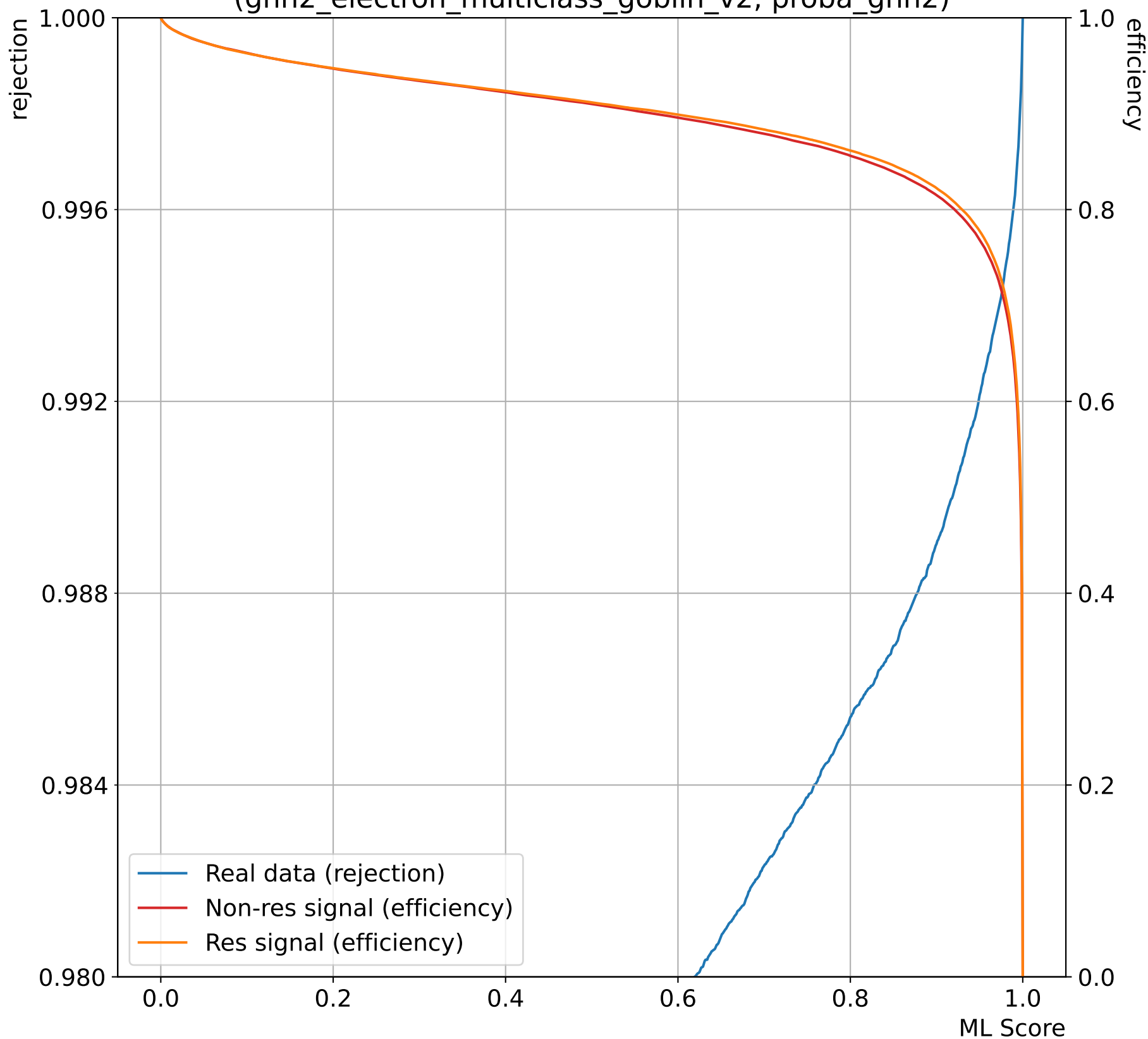
Efficiency in USR/rejection in NN1TRB, high q^2 (gnn2_electron_multiclass_goblin_v2, proba_gnn2)
