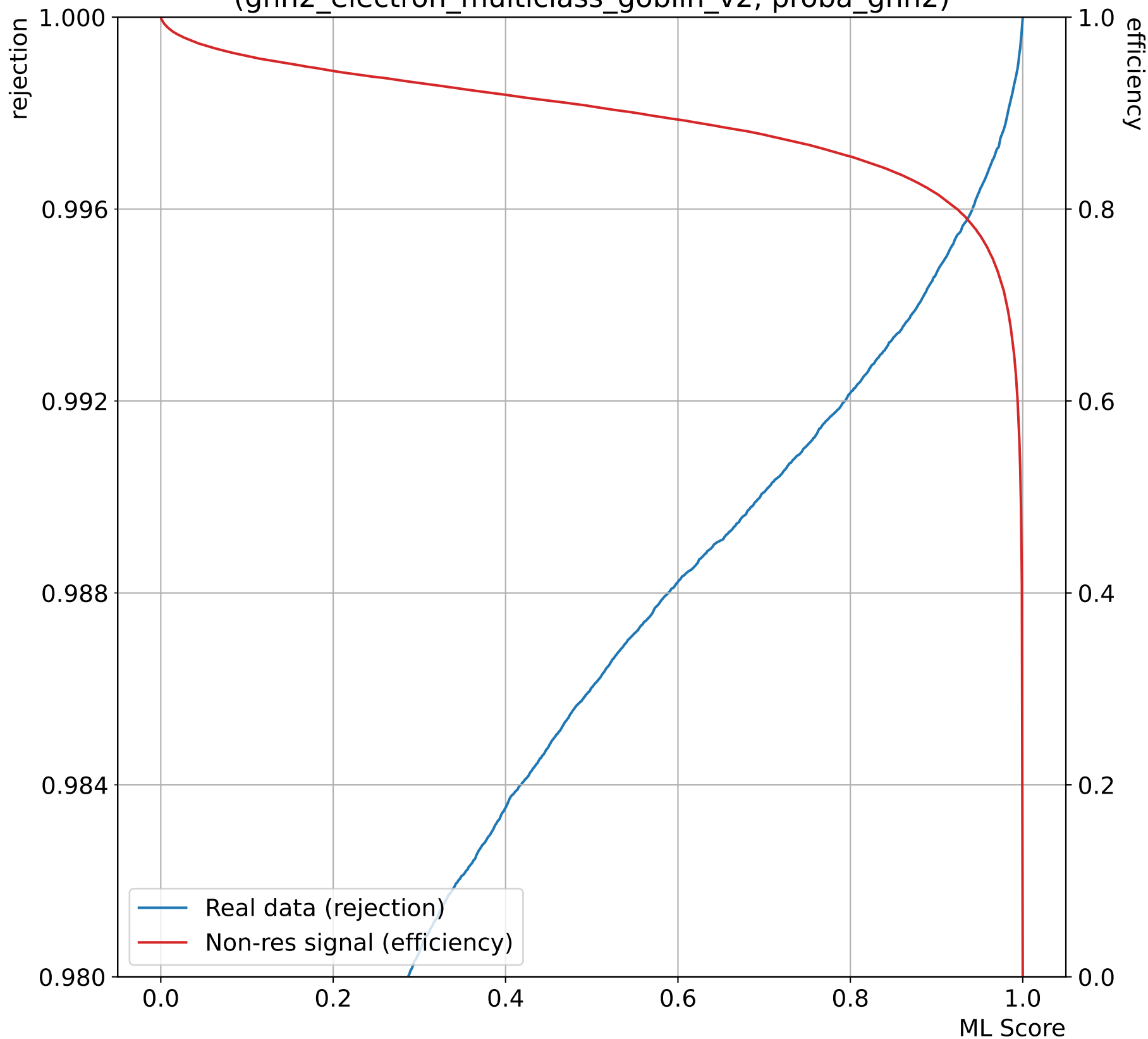
Efficiency in USR/rejection in NN1TRB, low q^2 (gnn2_electron_multiclass_goblin_v2, proba_gnn2)
