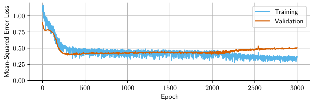
Innovation Driven LSTM Loss
