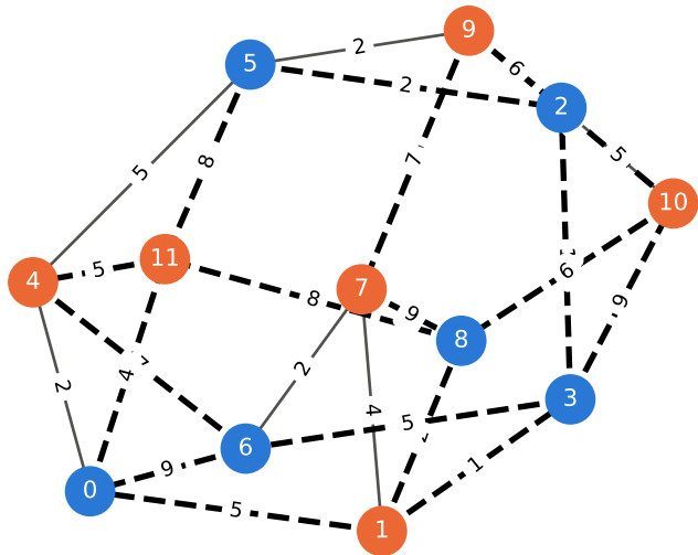
Gurobi: maximum cut = 100 (dashed edges)
