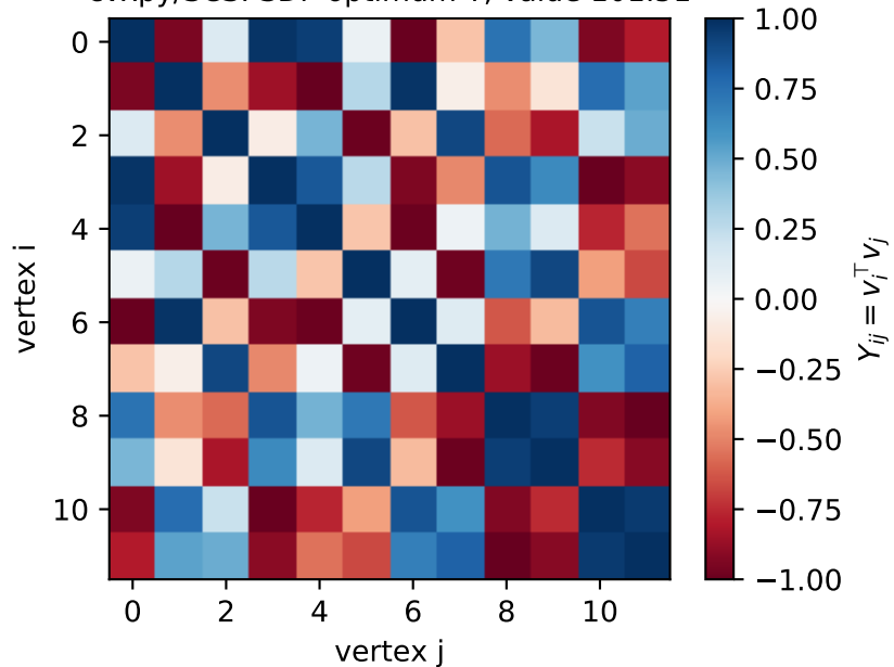
cvxpy/SCS: SDP optimum Y, value 101.51
