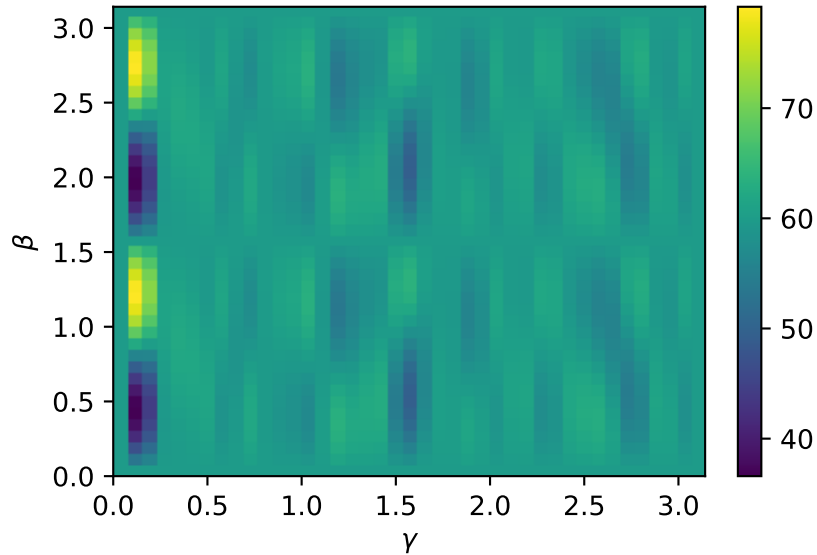
cold-start QAOA, p = 1 : \langle \text{cut} \rangle(\beta, \gamma)
