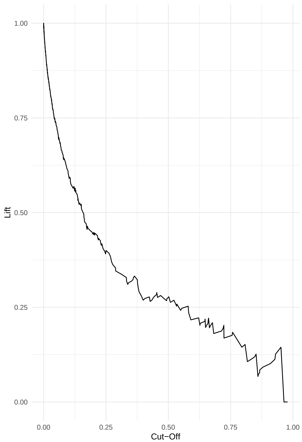
Lift Chart
