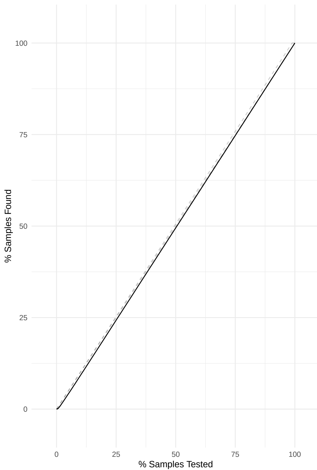
Cumulative Gain
