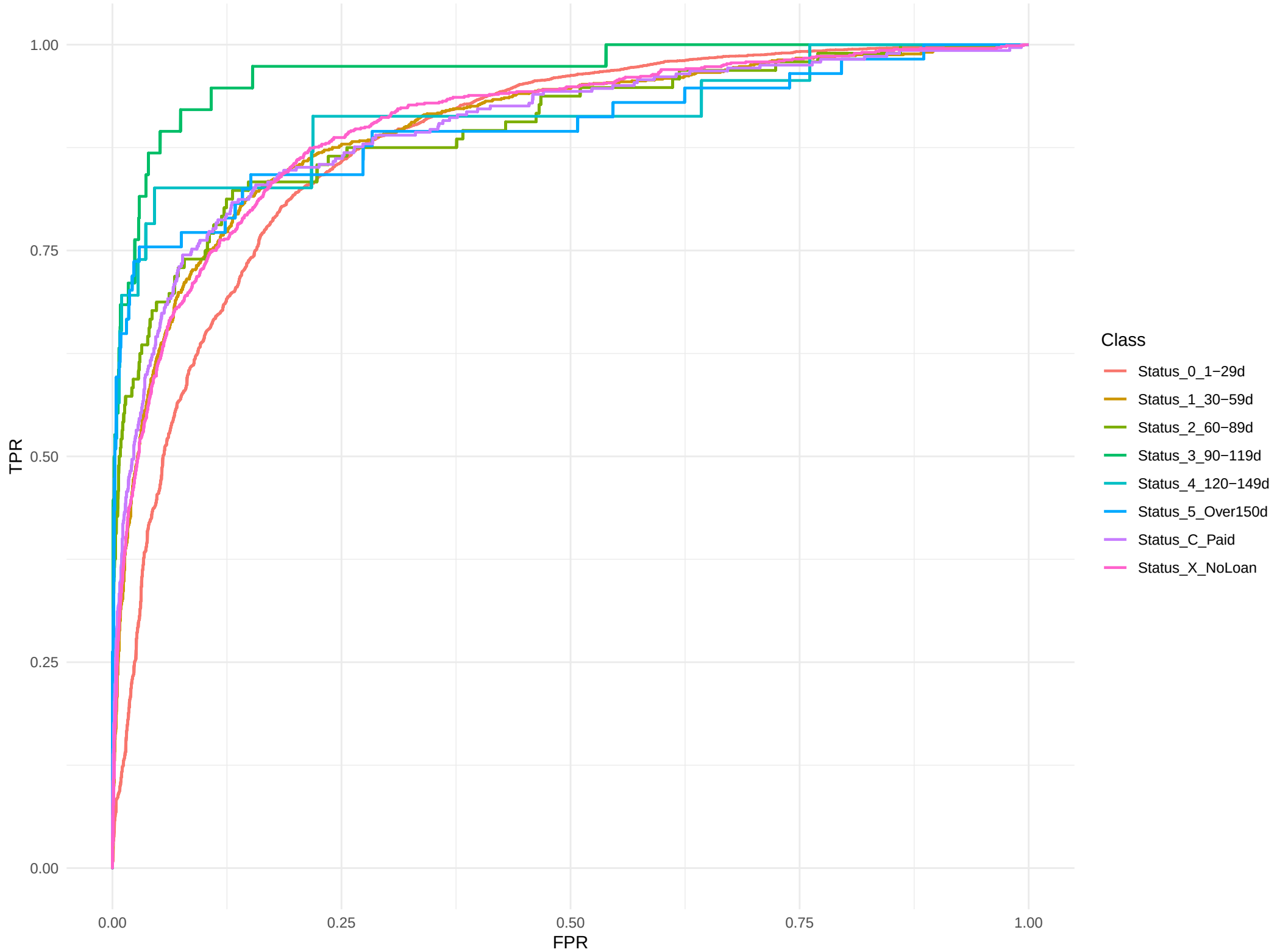
ROC Curves (Three-Stage Hierarchical Reconstruction)
