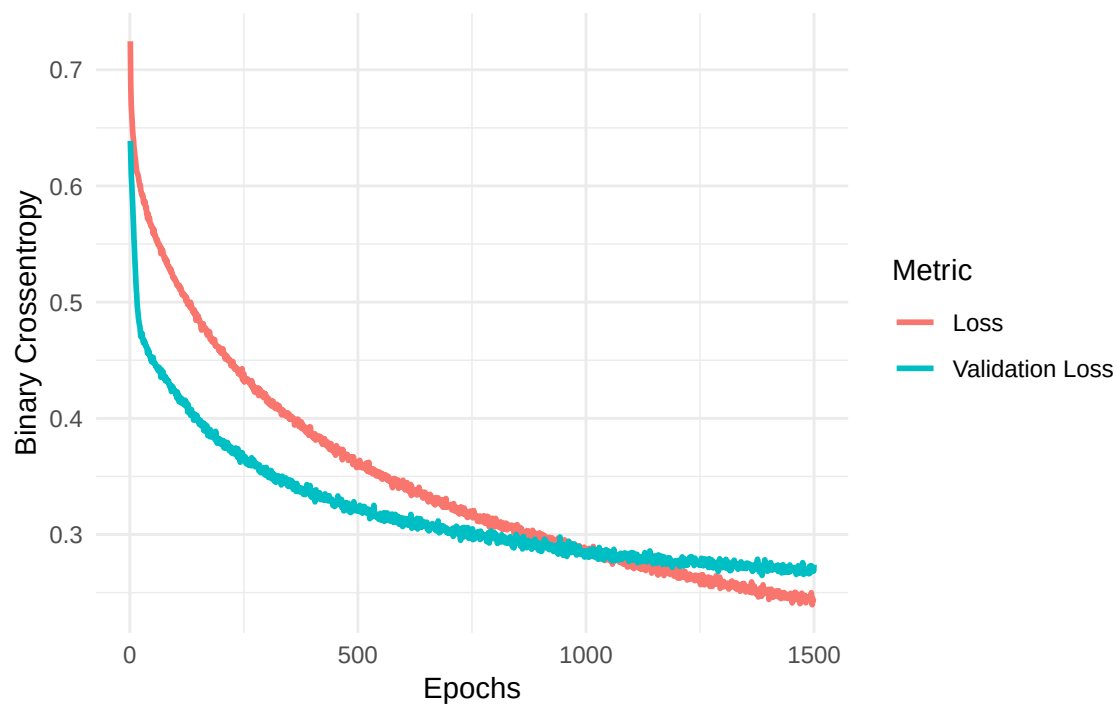
Learning Curve: Loss
