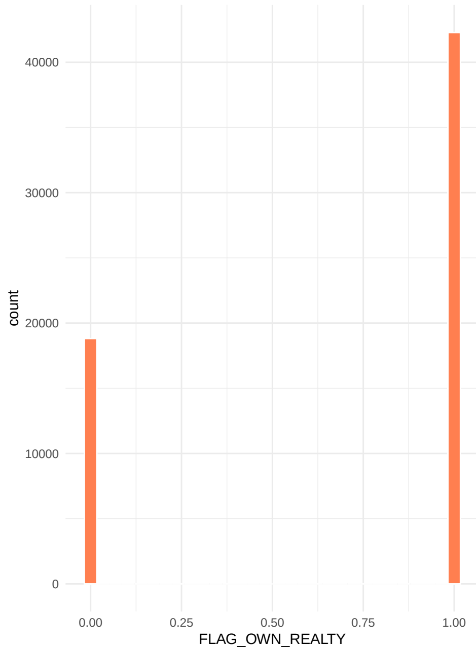
Distribution: FLAG_OWN_REALTY
