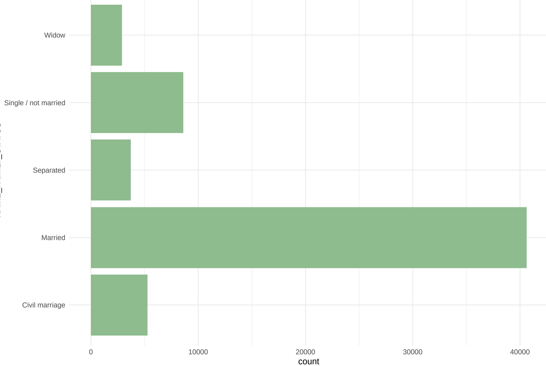
Frequency: NAME_FAMILY_STATUS
