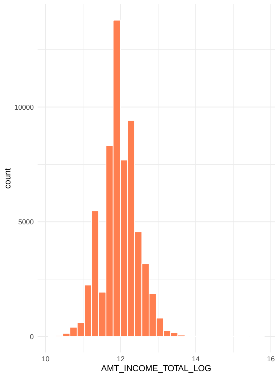
Distribution: AMT_INCOME_TOTAL_LOG
