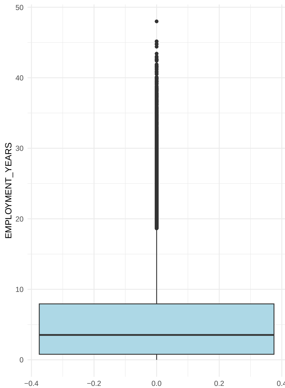
Outliers: EMPLOYMENT_YEARS
