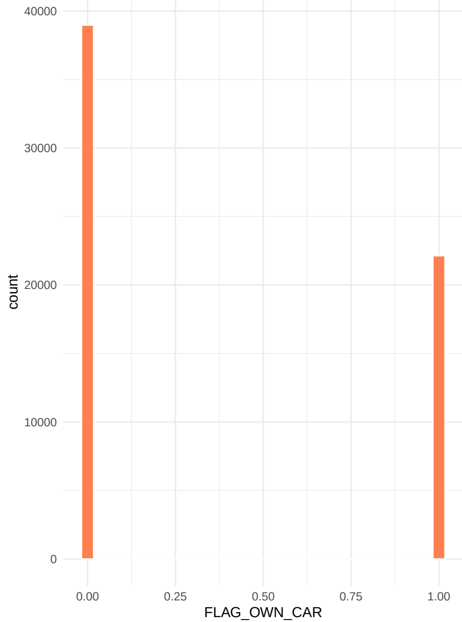
Distribution: FLAG_OWN_CAR
