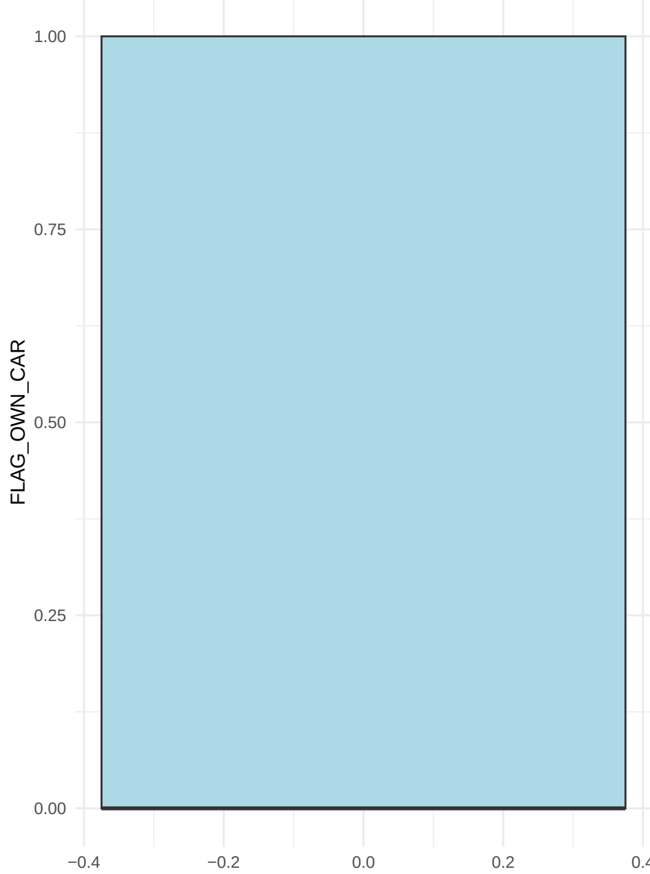
Outliers: FLAG_OWN_CAR
