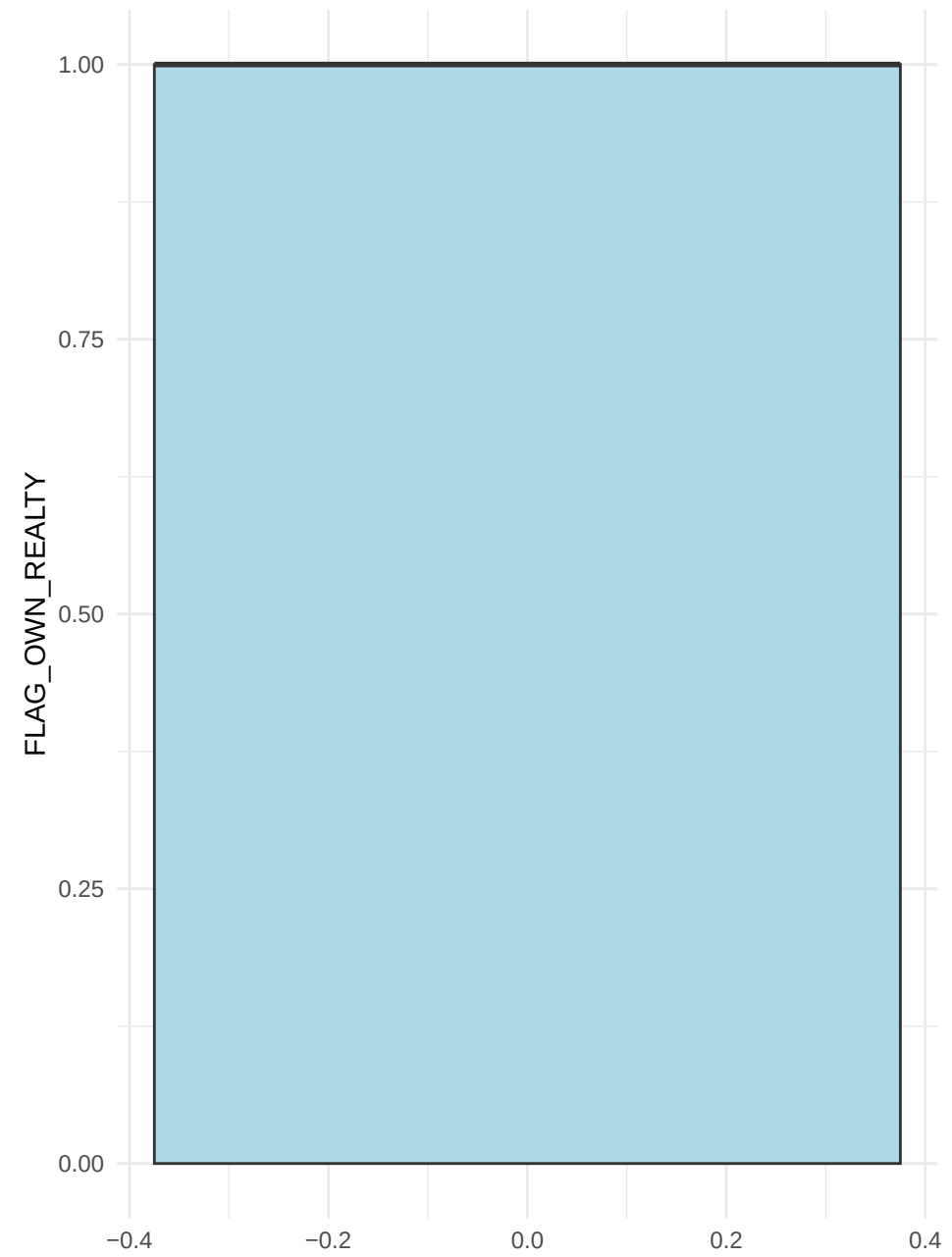
Outliers: FLAG_OWN_REALTY
