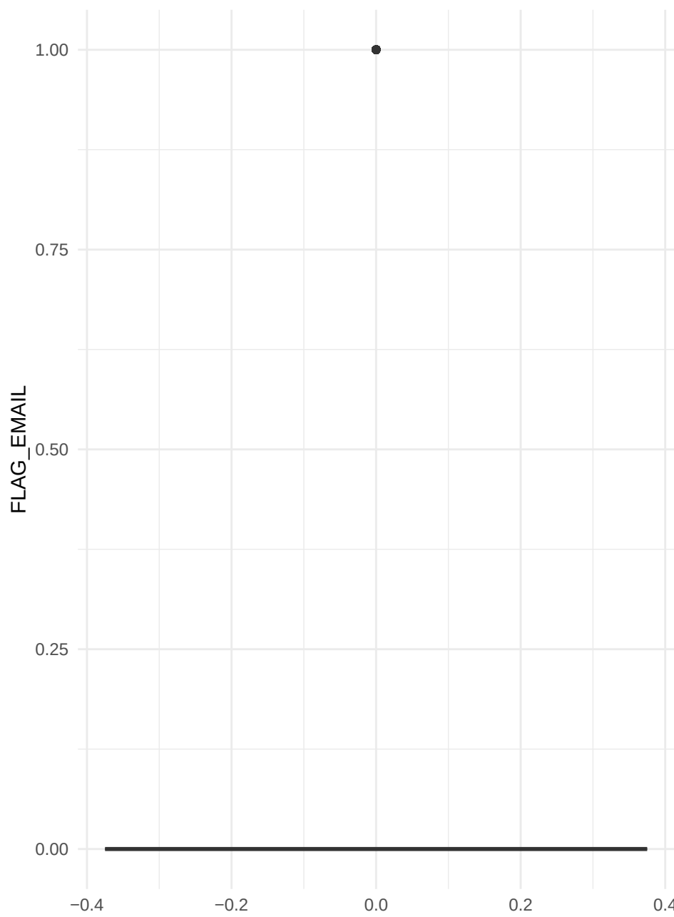
Outliers: FLAG_EMAIL
