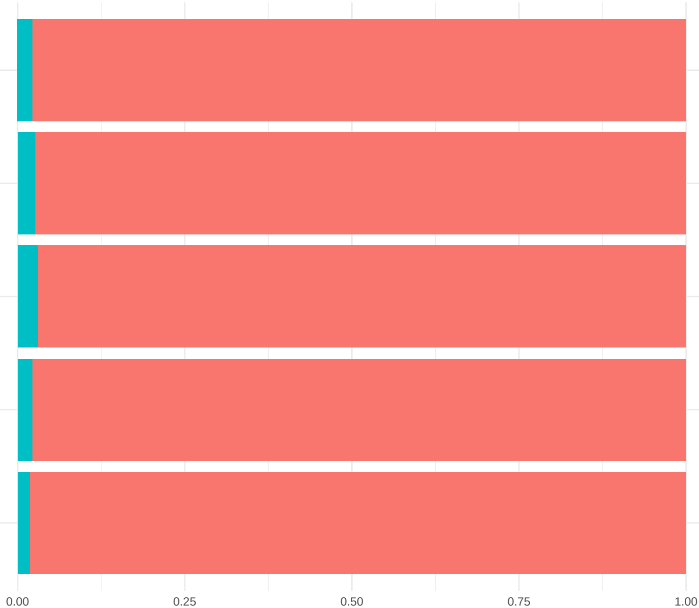
Target Proportion by NAME_FAMILY_STATUS
