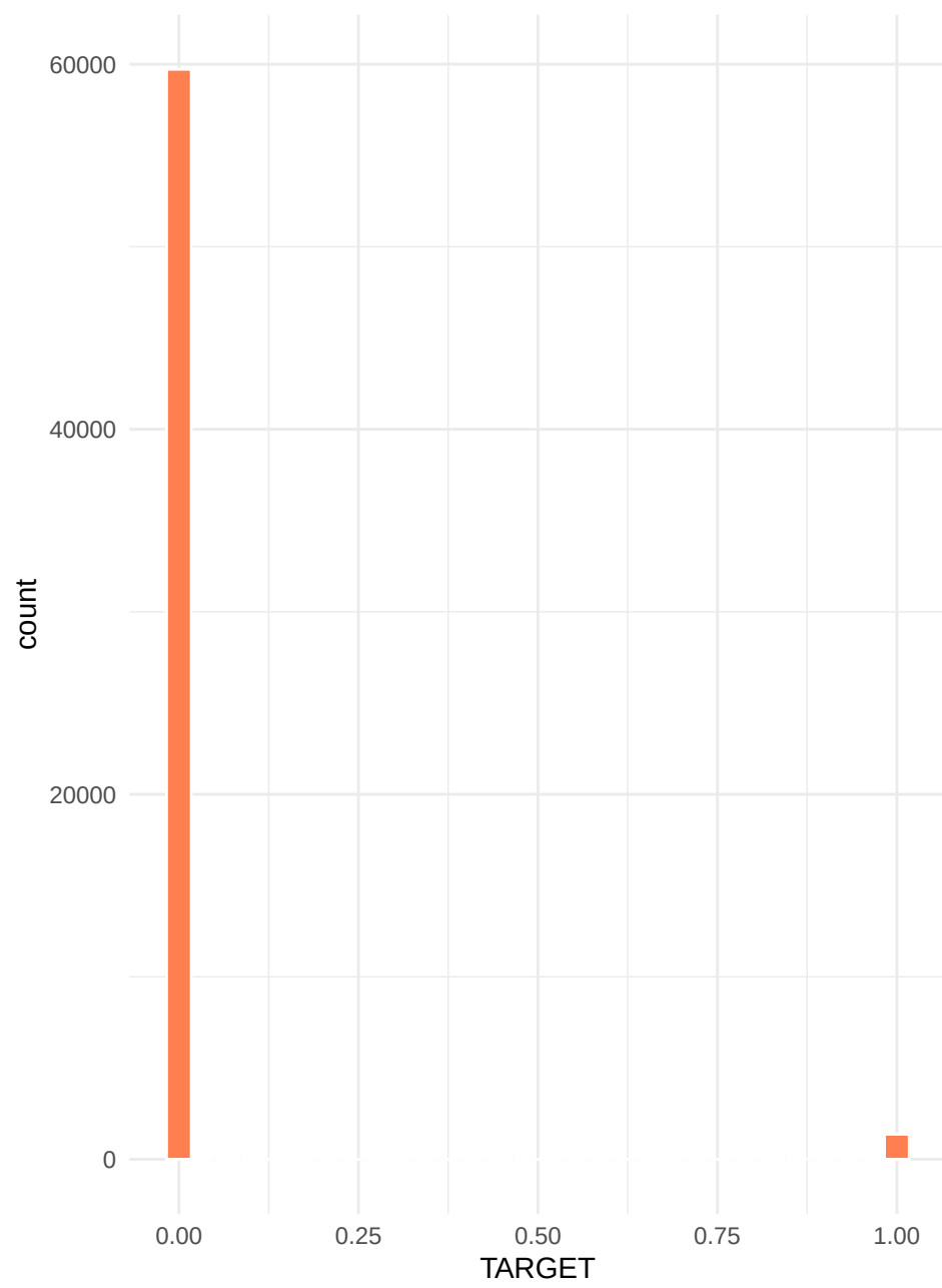
Distribution: TARGET
