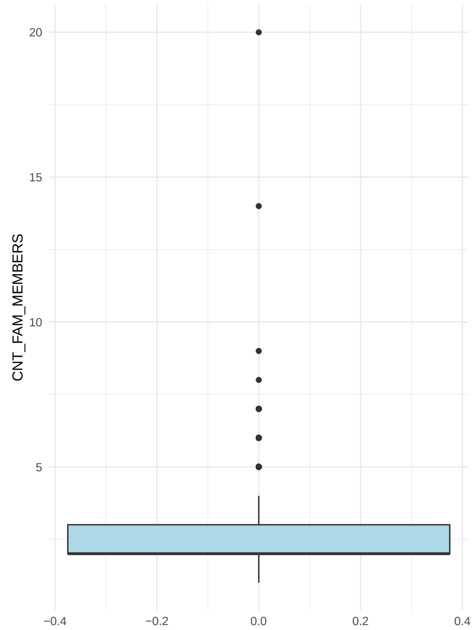
Outliers: CNT_FAM_MEMBERS
