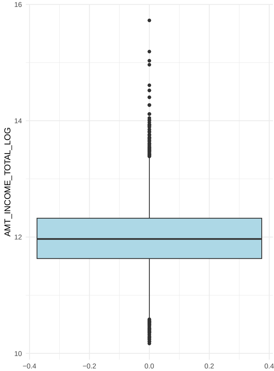
Outliers: AMT_INCOME_TOTAL_LOG
