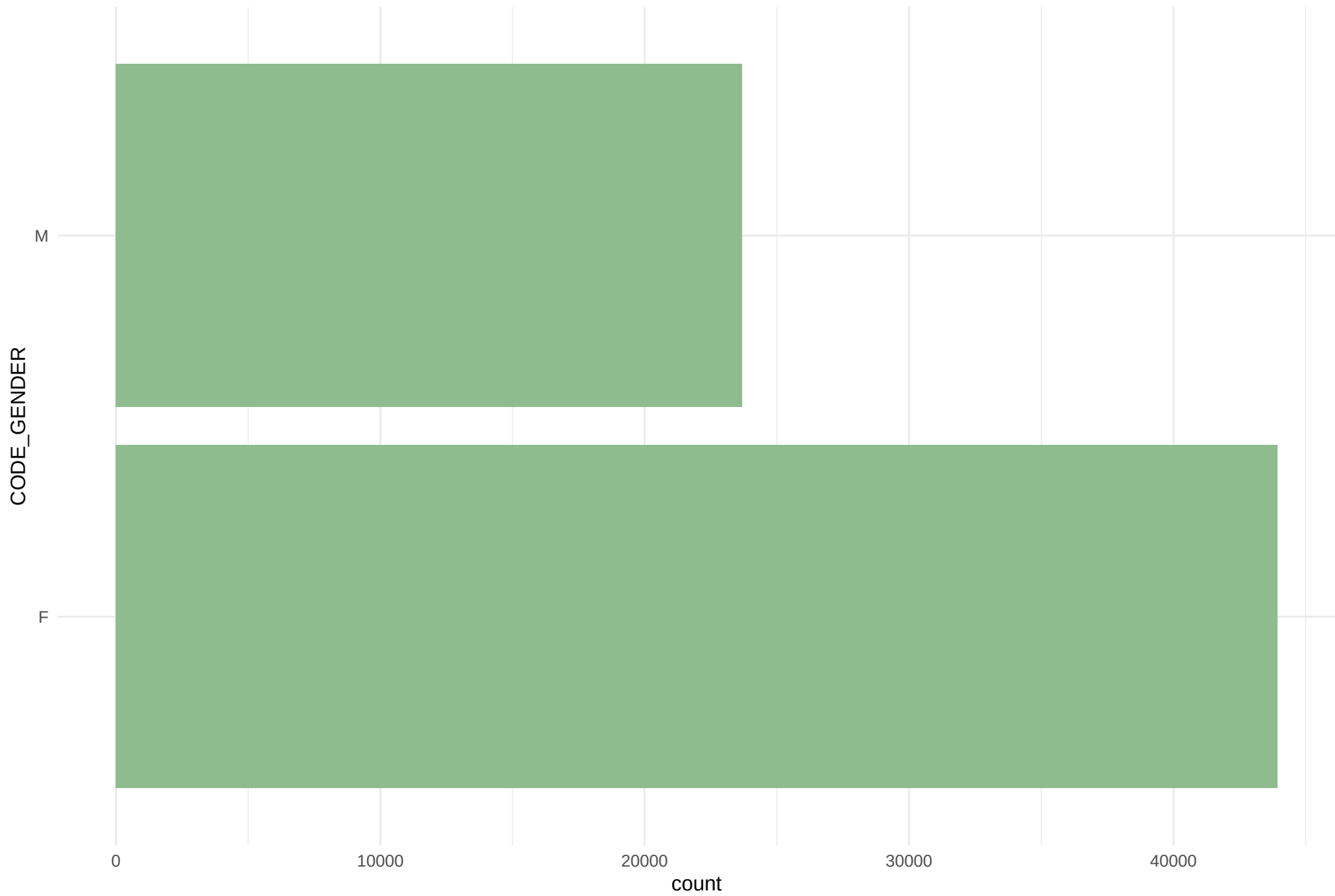
Frequency: CODE_GENDER
