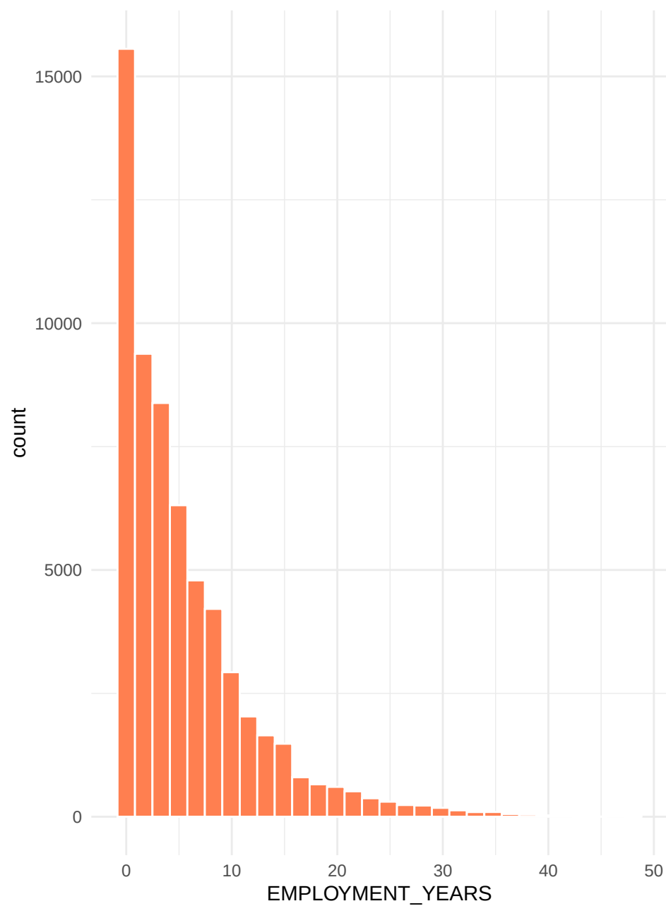
Distribution: EMPLOYMENT_YEARS
