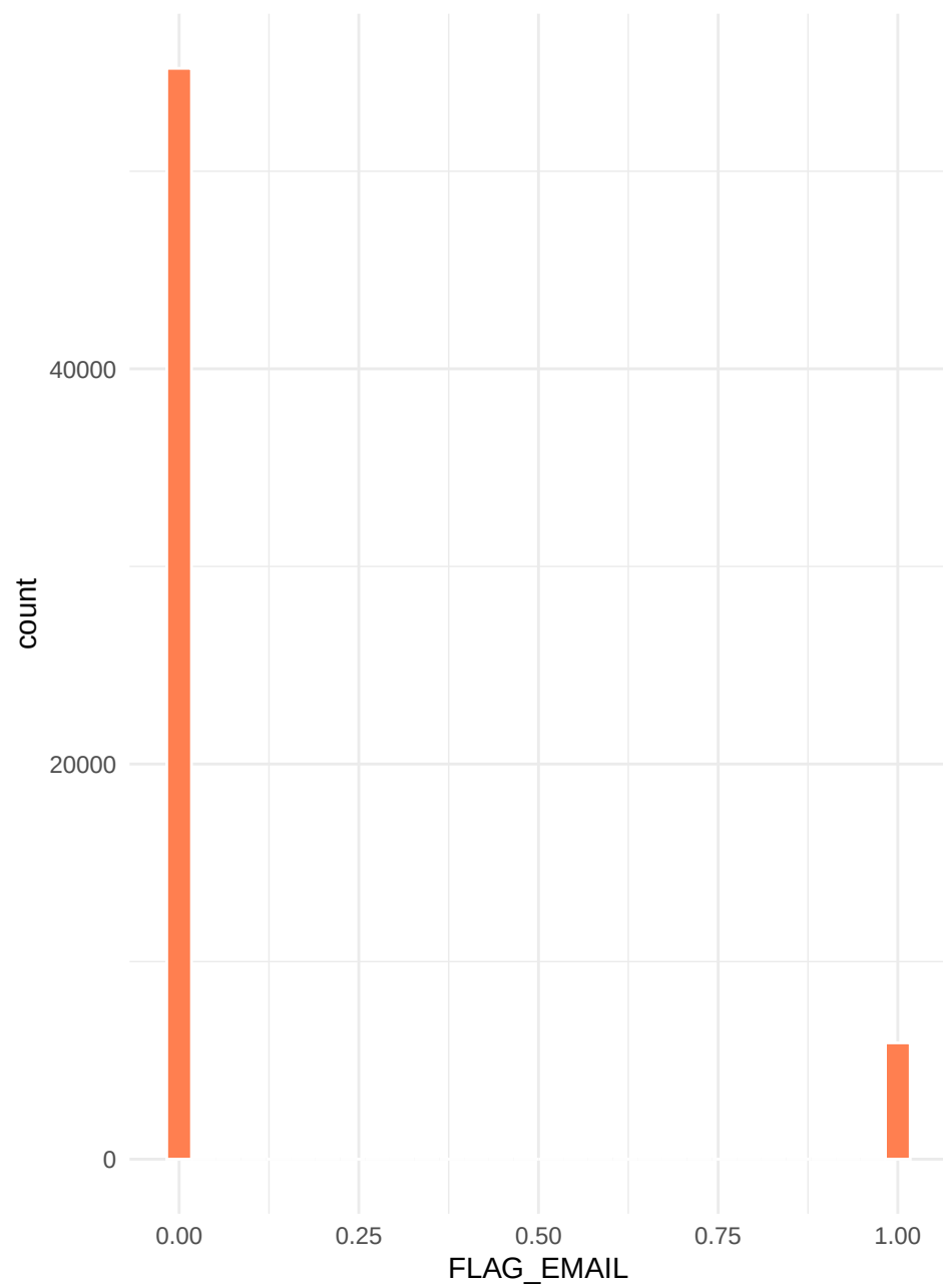
Distribution: FLAG_EMAIL
