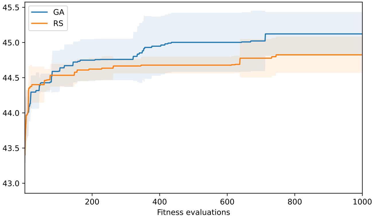
Best-so-far validation accuracy (%)
