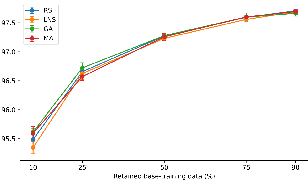
Best validation accuracy (%)
