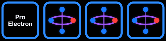
Pro Electron pro-electron
