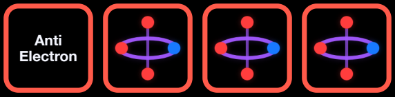
Anti Electron anti-electron
