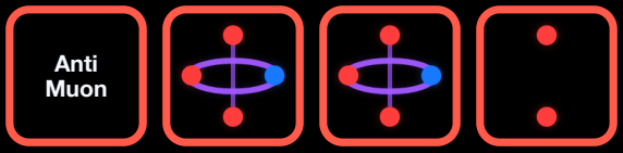
Anti Muon anti-muon
