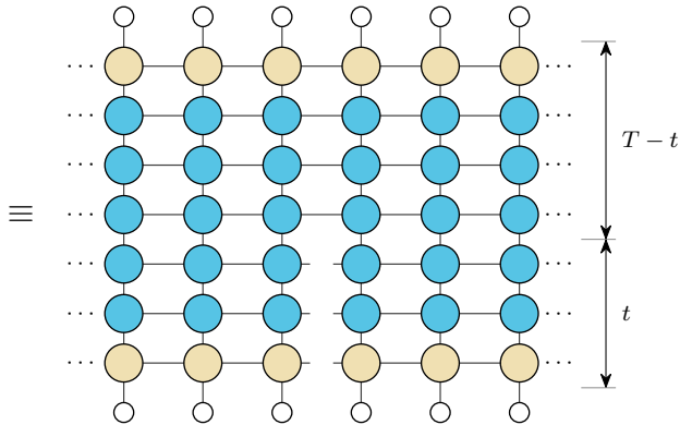
(b) the tensor network
