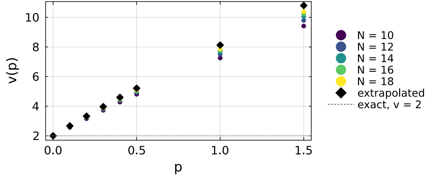
Figure 5: The sound velocity grows with the NNN coupling. v(p) at \lambda = 1 , from the equilibrium dispersion of periodic rings of N = 10 to 18 sites (coloured circles), together with the values extrapolated to the thermodynamic limit (black diamonds), which are the ones used throughout. The dotted line marks the exact Ising value v = 2 at p = 0 .
