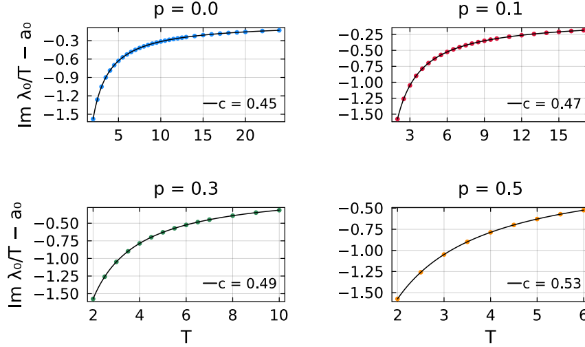
Figure 10: Central charge from the phase of the leading eigenvalue. Fits of Eq. (6) to \text{Im } \lambda_0/T at each coupling. The fitted constant a_0 is subtracted to isolate the time-dependent contribution, whose curvature determines the central charge reported in each legend.
