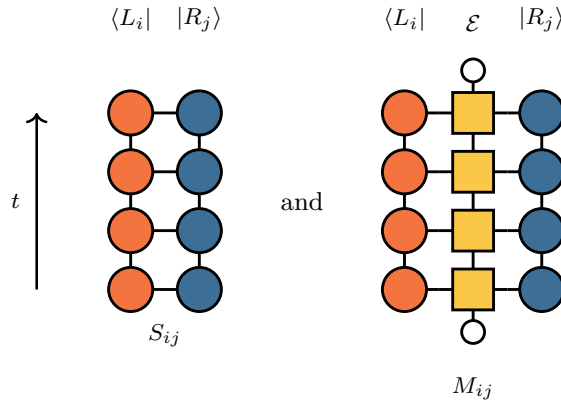
Figure 20: The two projected matrices. Contractions defining the k \times k matrices of Eq. (19). Each tMPS forms a column, while \mathcal{E} is the corresponding column of the space–time network closed at both ends by the product state (small open circles). The left chain enters directly as a bra, without complex conjugation.
