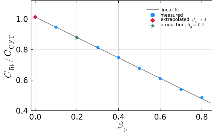
Figure 24: Fitted phase coefficient as a function of the cooling regulator. Integrable-point results, expressed as a fraction of the value predicted by Eq. (6). All points use the same fitting window and differ only in N_\beta . The dependence is approximately linear and extrapolates to within a few per cent of the prediction as \beta_0 \rightarrow 0 . At the production value \beta_0 = 0.2 , the coefficient lies approximately 12% below the prediction, showing the contribution of the finite regulator to the deficit.
