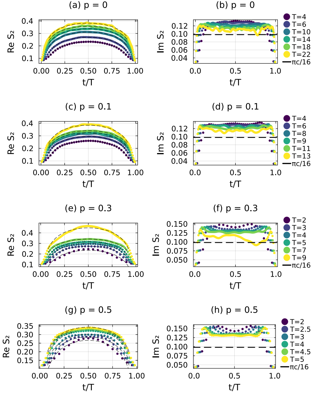
Figure 23: Generalised temporal entropy at the four couplings. Each row spans the entropy window for one coupling in Table 1. The left panels show \text{Re } S_2 as a function of t/T . The dashed curves show Eq. (G.1) for c = \frac{1}{2} , with the offset and correction amplitude fitted separately to each profile. The right panels show \text{Im } S_2 ; the dashed line marks \pi c/16 = 0.098 , and the displacement from this value is the finite-time correction.
