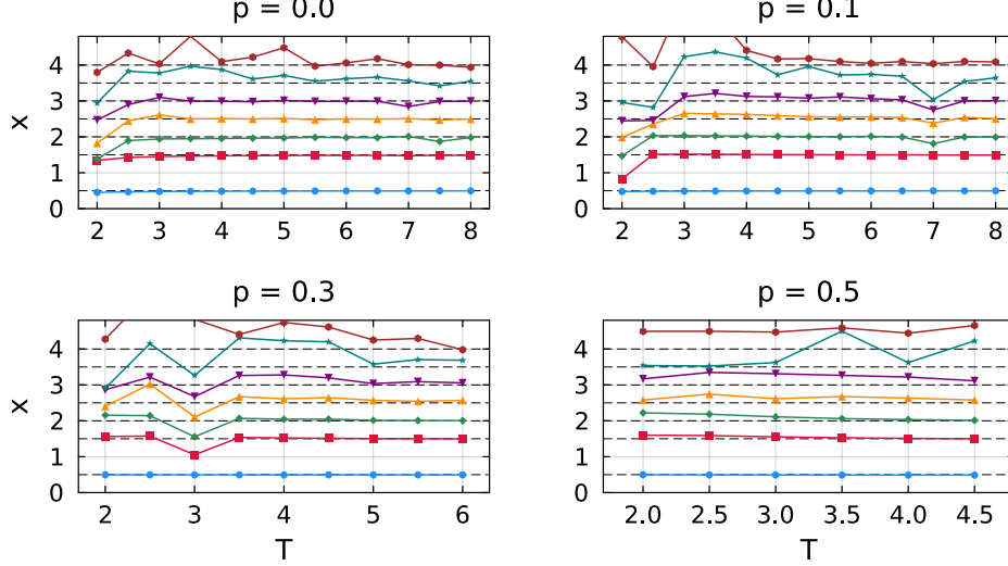
Figure 11: Boundary dimensions as a function of evolution time. The seven leading dimensions at each coupling are obtained from the phase gaps through Eq. (7), ordered by increasing phase distance from \mu_0 , and resolved with k = 8 . The dashed lines mark the predicted values \frac{1}{2} , \frac{3}{2} , 2 , \frac{5}{2} , 3 , \frac{7}{2} , and 4 . The free boundary condition selects two towers: the identity tower contains the integer values, while the energy tower contains the half-integer values (Appendix G.2).
