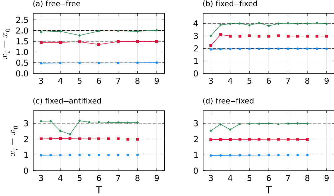
Figure 25: Boundary towers at the integrable point. The three leading spacings x_i - x_0 are obtained from Eq. (7); dashed lines mark the predicted values. (a) Free--free. (b) Fixed--fixed. (c) Fixed--antifixed. (d) Free--fixed. The two mixed cases have the same spacings and are distinguished by the tower positions in Table 11.
