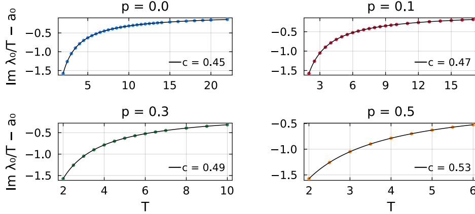
Figure 10: Central charge from the phase of the leading eigenvalue. Fits of Eq. (6) to \text{Im } \lambda_0/T at each coupling. The fitted constant a_0 is subtracted to isolate the time-dependent contribution, whose curvature determines the central charge reported in each legend.
