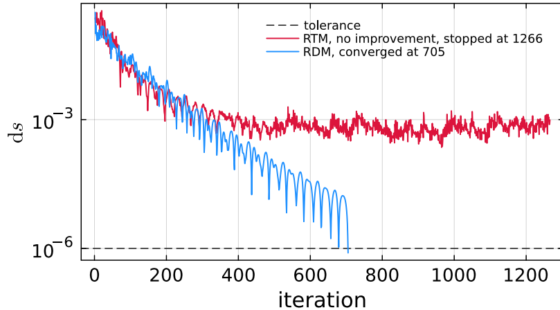
Figure 21: Termination of the single-vector iteration. The change ds as a function of iteration number at p = 0 and T = 12 , for both truncation schemes started from the same random state. With RTM truncation, ds reaches a floor above the tolerance and the no-improvement rule terminates the run. With RDM truncation, it crosses the tolerance. The two calculations return leading eigenvalues that agree within 0.01%.
