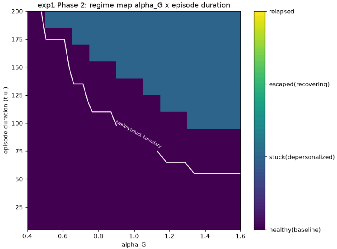
Figure 1: Figure 1: Collapse regime map over the full \alpha G \times \text{episode-duration} grid — 214 healthy / 98 stuck cells, zero intermediate outcomes; the transition is all-or-nothing at the horizon.
