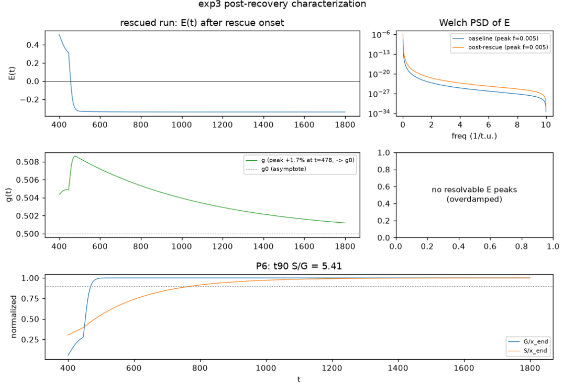
Figure 5: Figure 5: Post-recovery characterization of a fully rescued run — E(t) after rescue onset with its Welch PSD, the g(t) overlay relaxing to g_0 (the transient is everything there is), no resolvable E peaks (overdamped), and the P6 recovery-lag inset.
