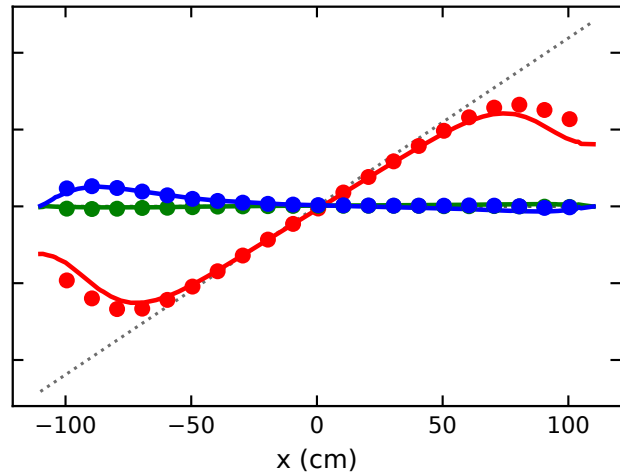
(b) Calibration-corrected COMSOL prediction
