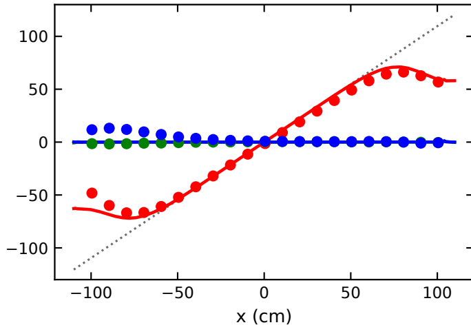
(a) Original COMSOL prediction
