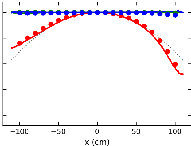
(b) COMSOL-derived currents
