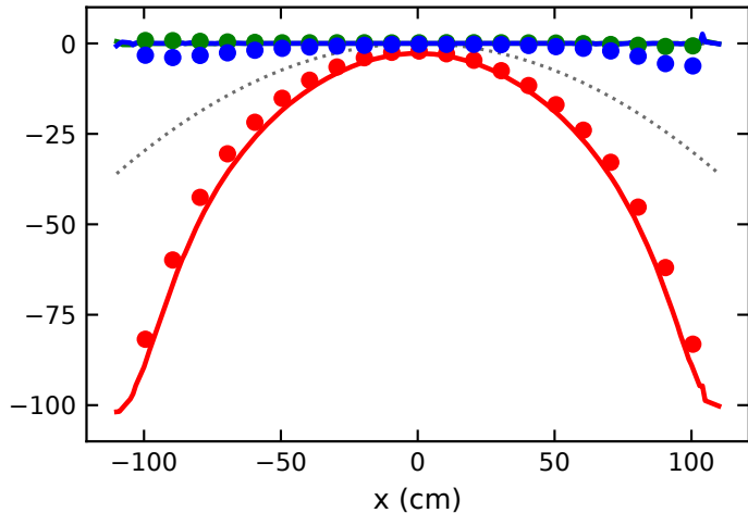
(a) Free-space-derived currents
