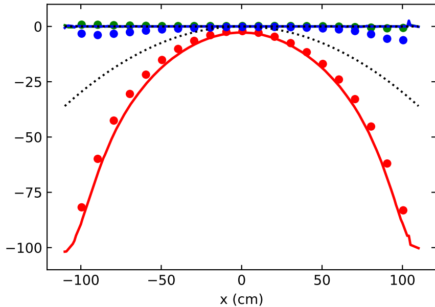
(a) Free-space-derived currents
