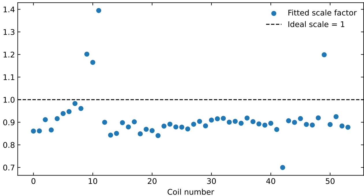
Fitted COMSOL scale factor
