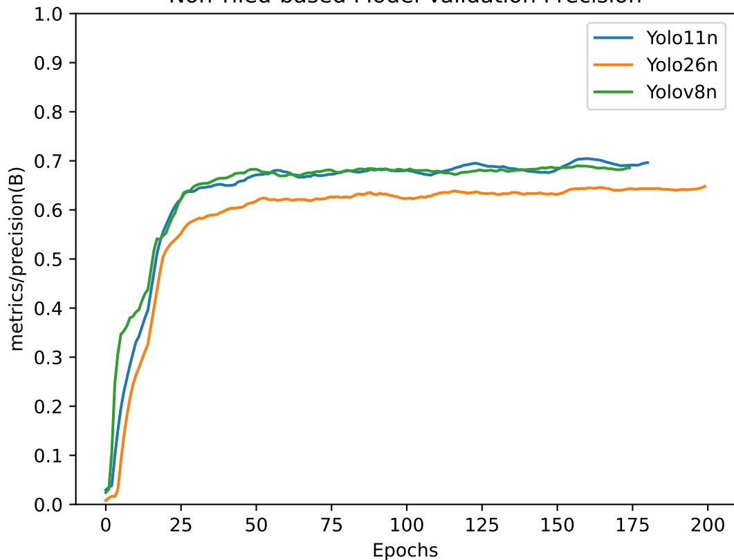
Non-Tiled-based Model Validation Precision
