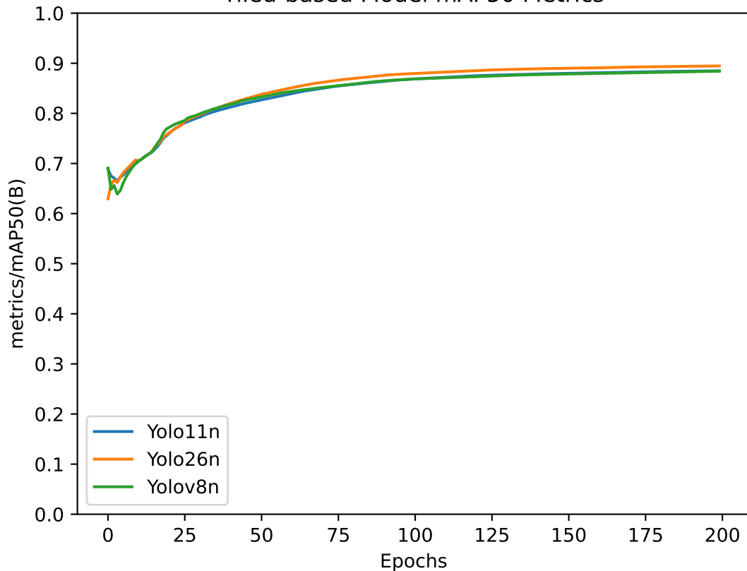
Tiled-based Model mAP50 Metrics
