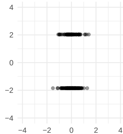
Residual vs. Predicted
