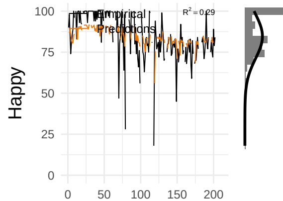
Empirical &amp; Predicted
