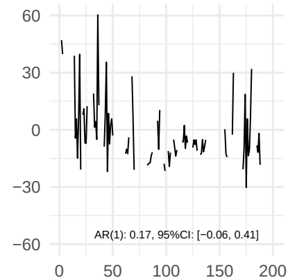
Residuals
