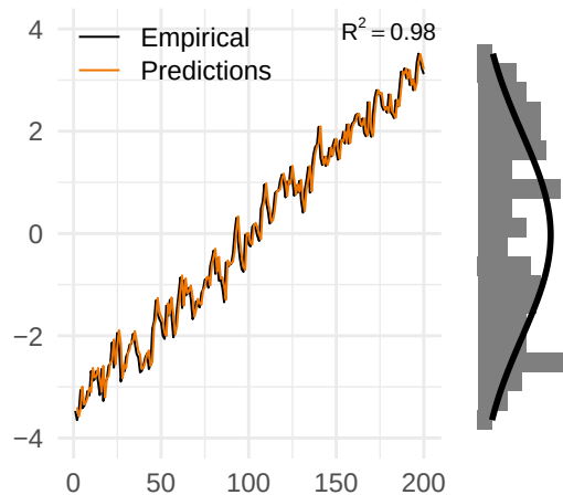
Switching/Non-Linear
