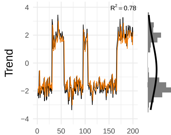
Switching/Non-Linear
