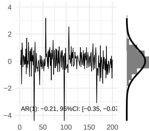
Residuals
