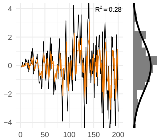
Changing Innovations
