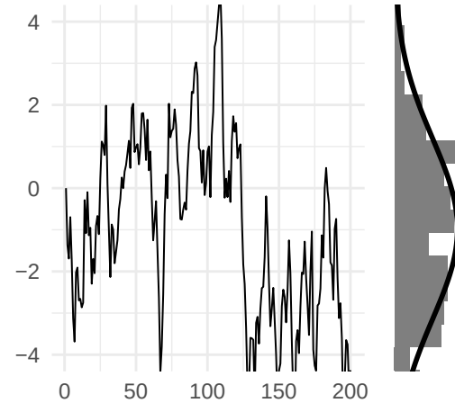
Simulated
