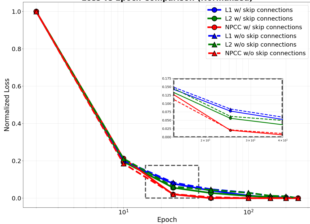
Loss vs Epoch Comparison (Normalized)
