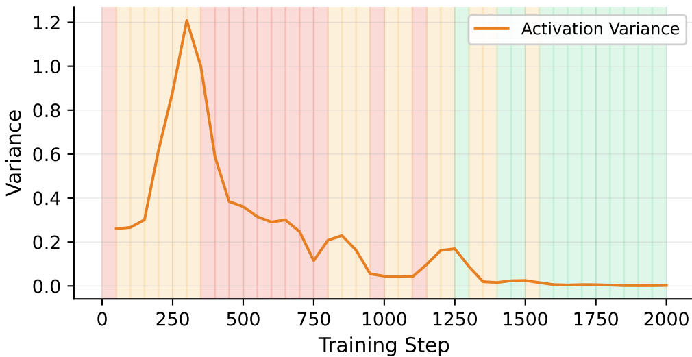
Activation Variance
