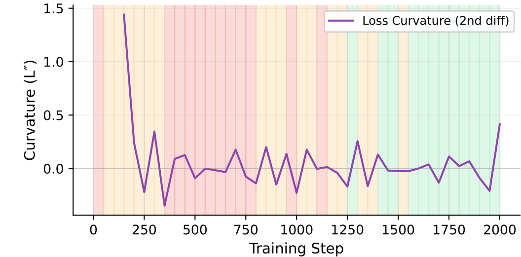
Loss Curvature
