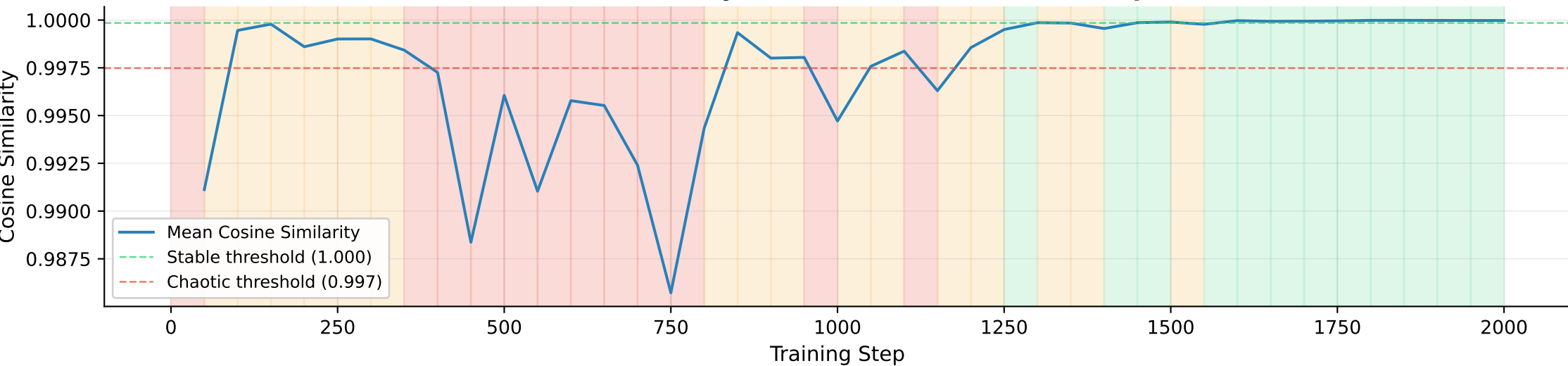
Activation Similarity Between Consecutive Checkpoints
