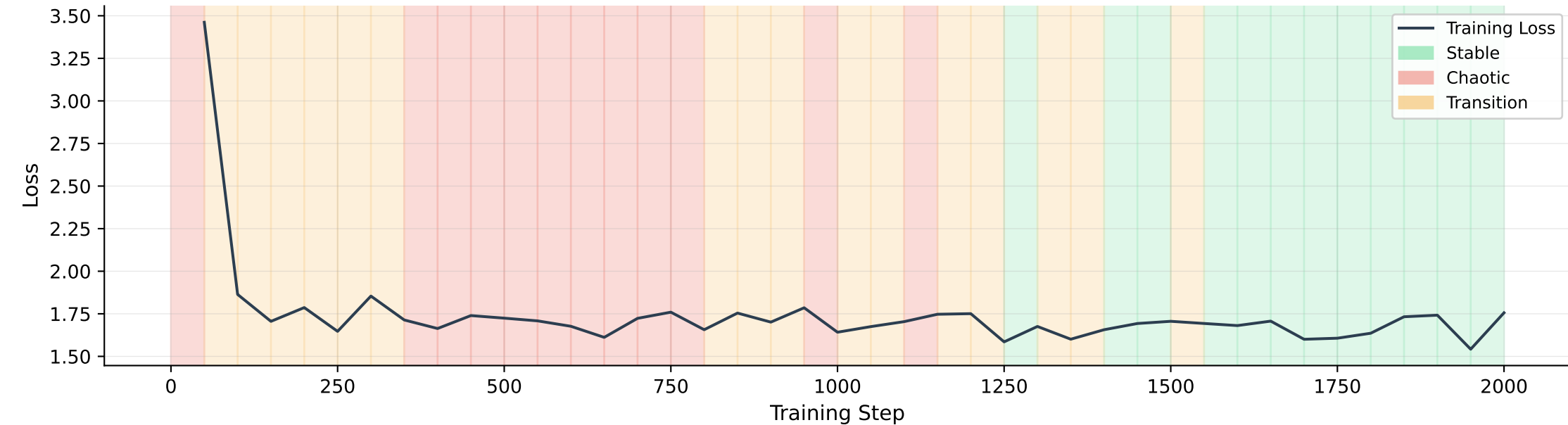
Training Loss with Regime Detection
